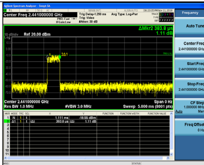
2-DH1
