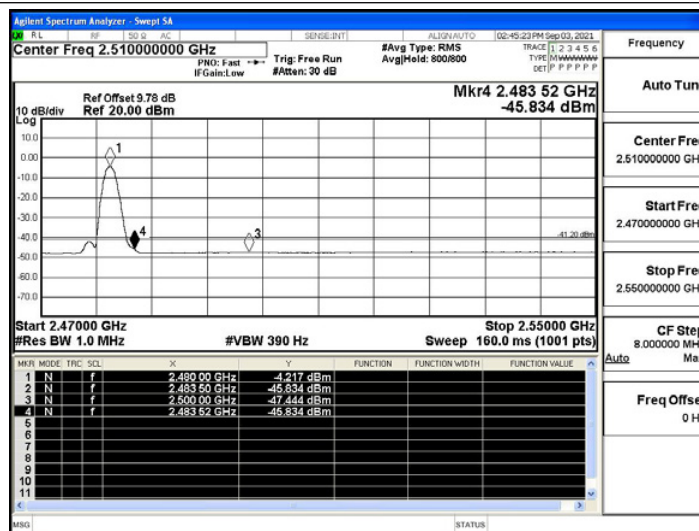
DH5_Ant1_High_2480_Peak
