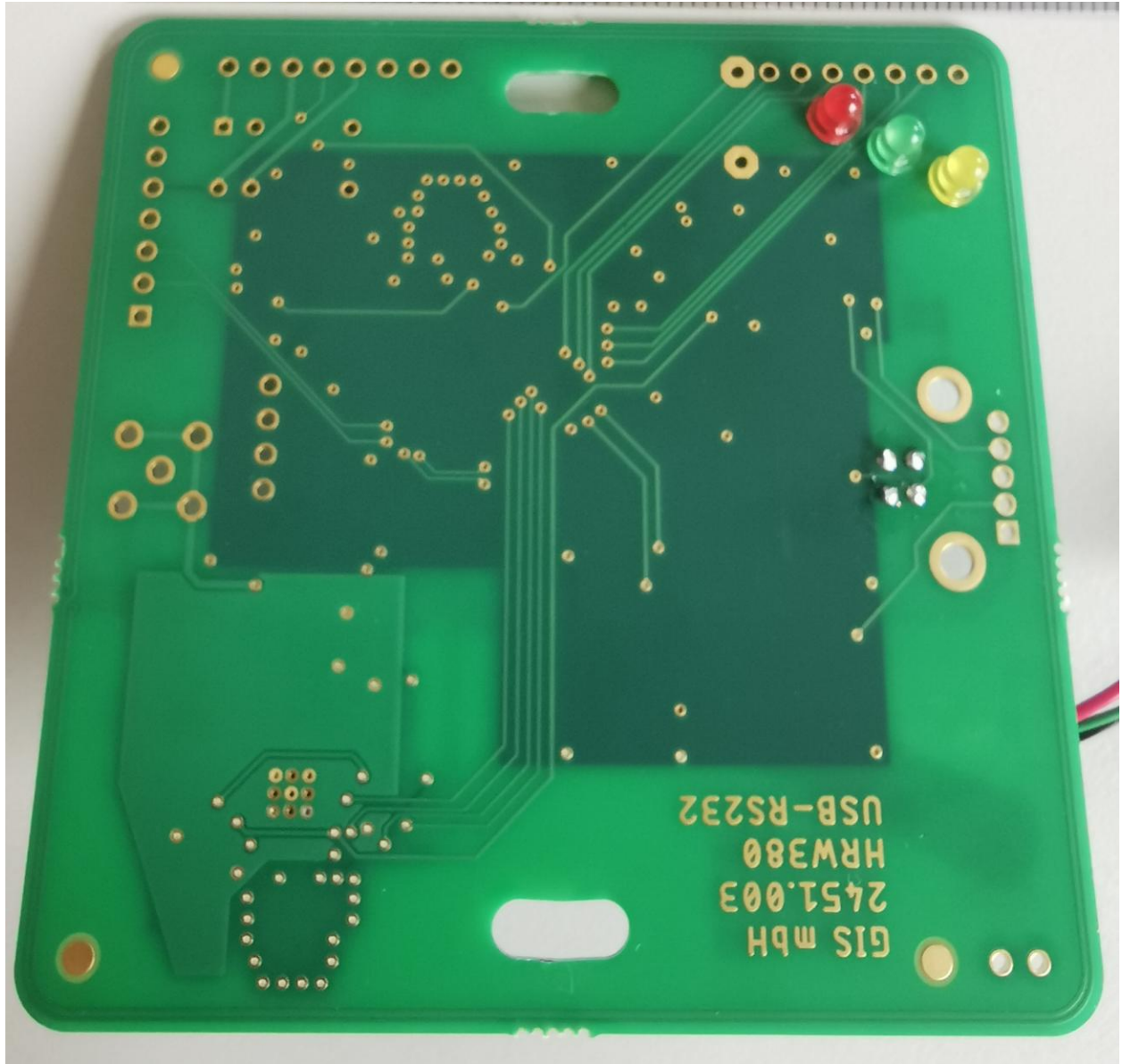
Figure 2: PCB Back
