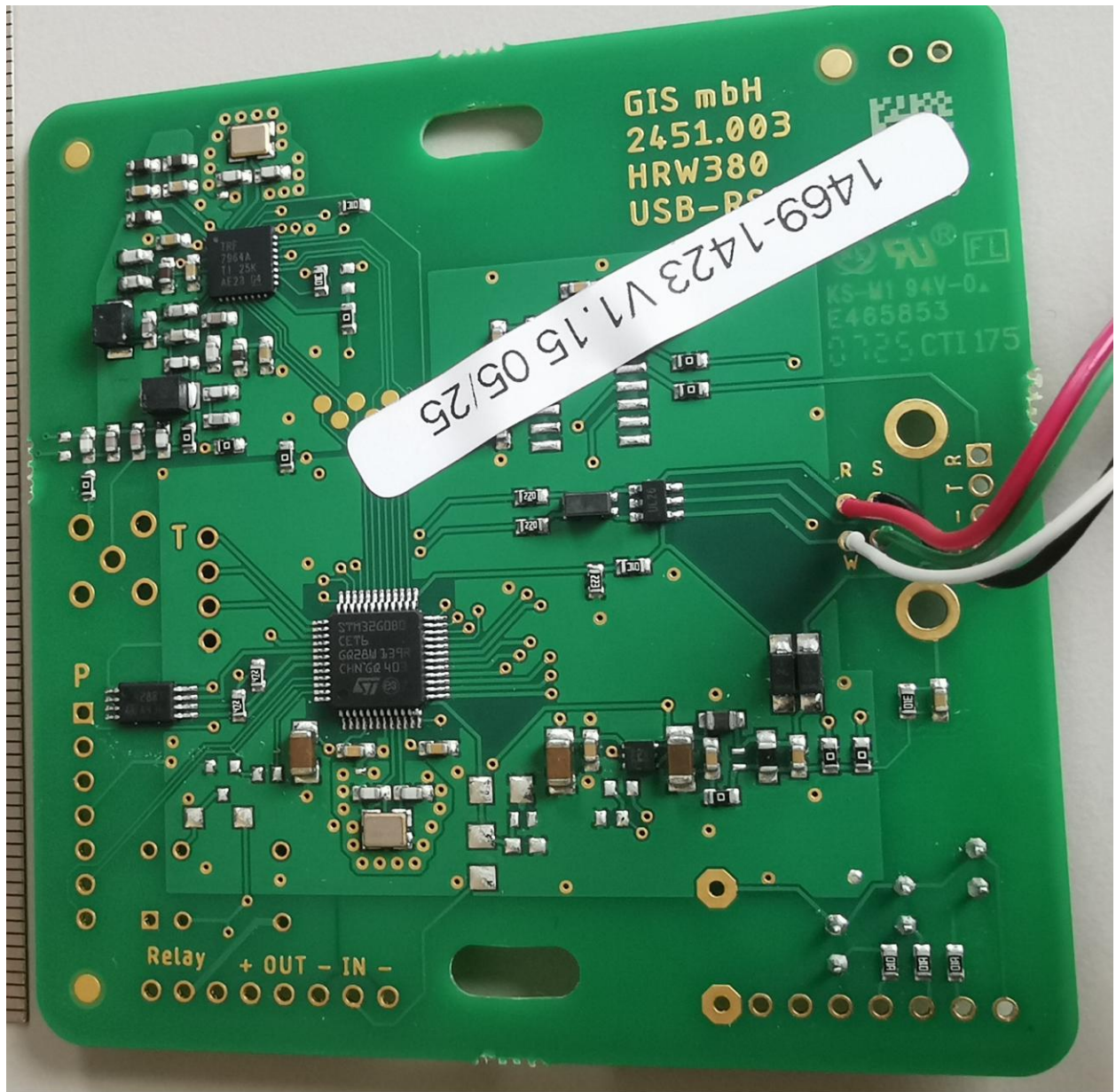
Figure 1: PCB Front
