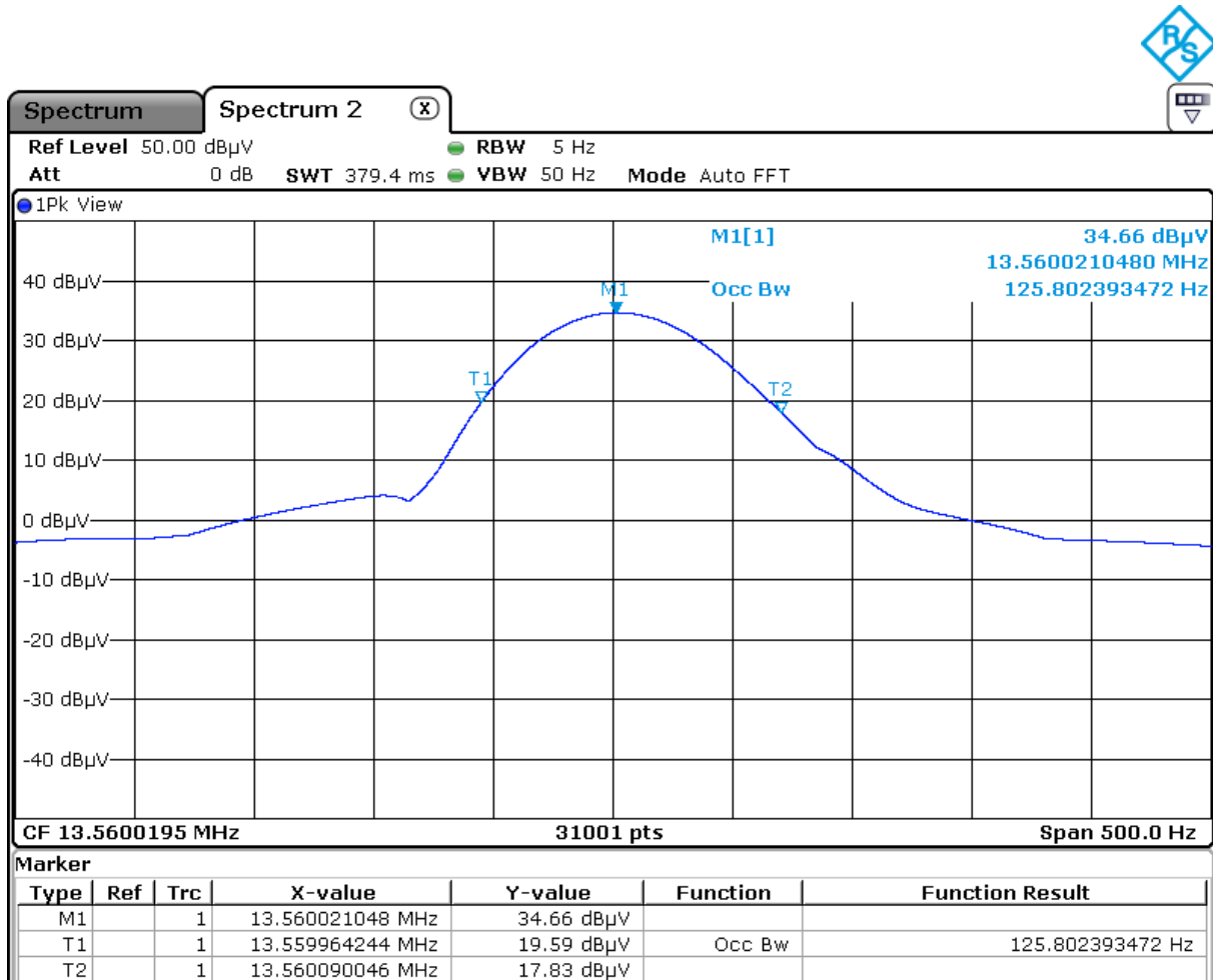
Figure 3 – 99 % Bandwidth
