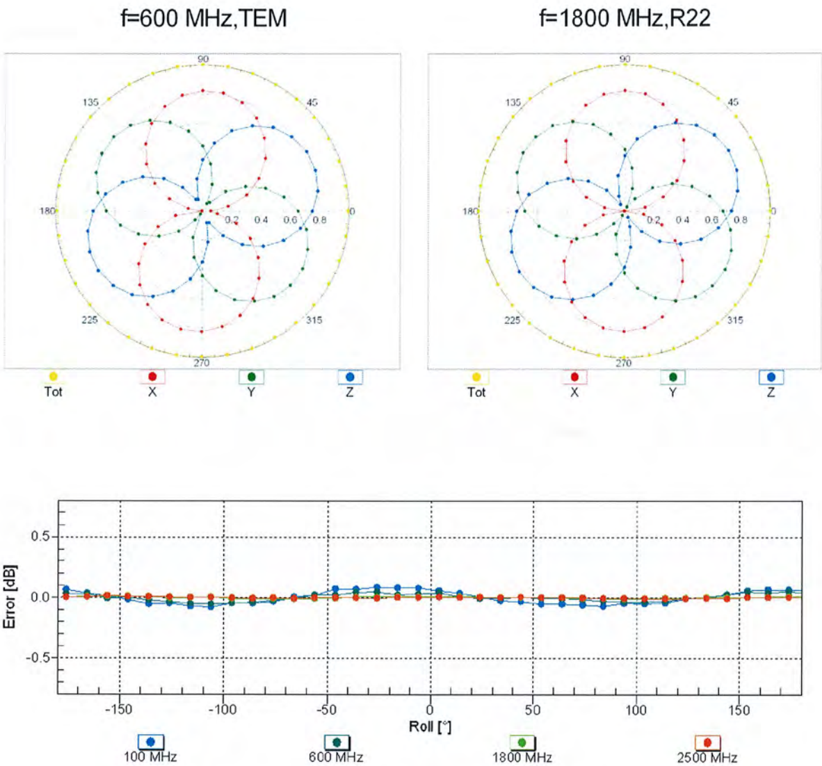
Uncertainty of Axial Isotropy Assessment: ± 0.5% (k=2)
