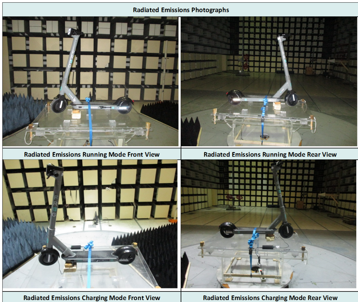
Radiated Measurement Setup below 18 GHz.
