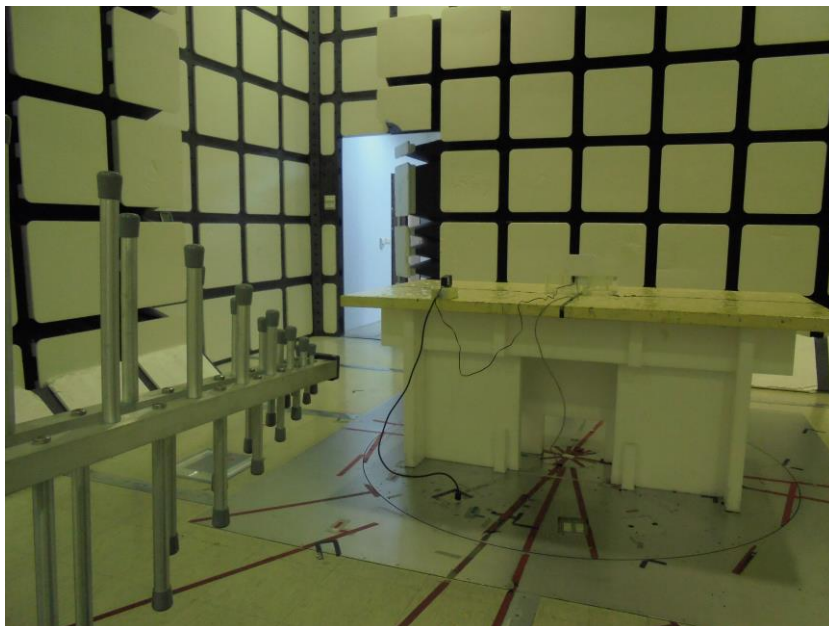
Below 1 GHz _ Rear View
