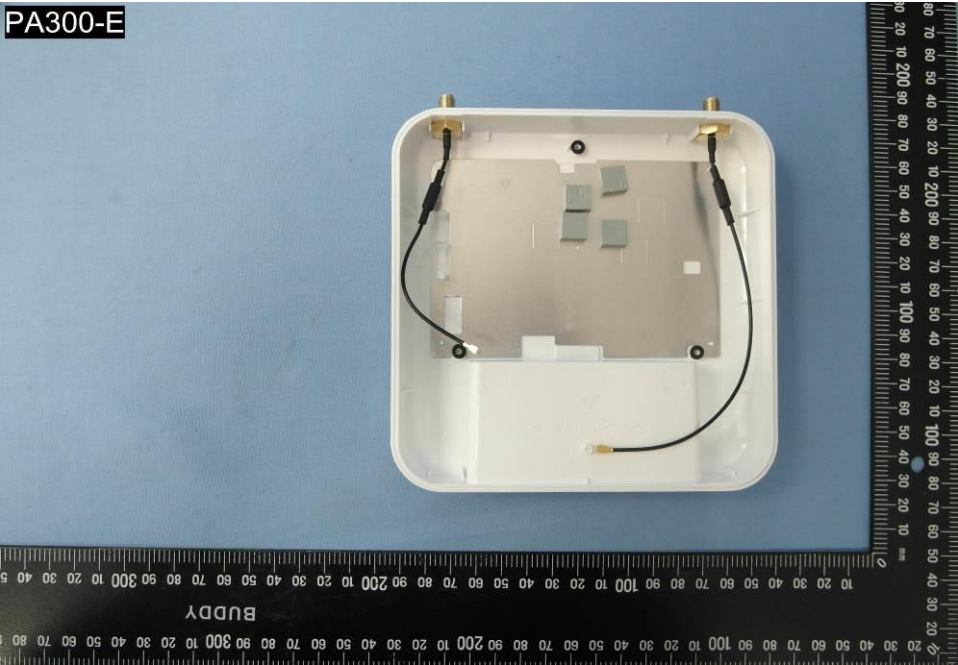
EUT Photo (23)
