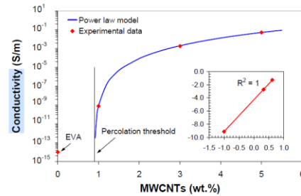
Figure 15. Variation of electrical conductivity as a function of MWCNT wt.% (Experimental data correspond to the optimum injection molding parameters).
