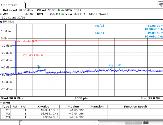
BLE_2M_Low_Channel
