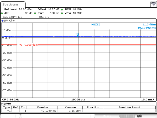
BLE_2M_Middle_Channel
