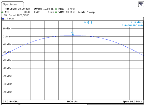
BLE_2M_Middle_Channel
