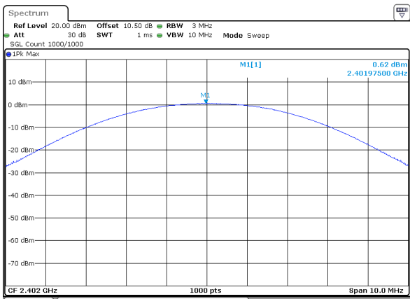
BLE_1M_Low_Channel
