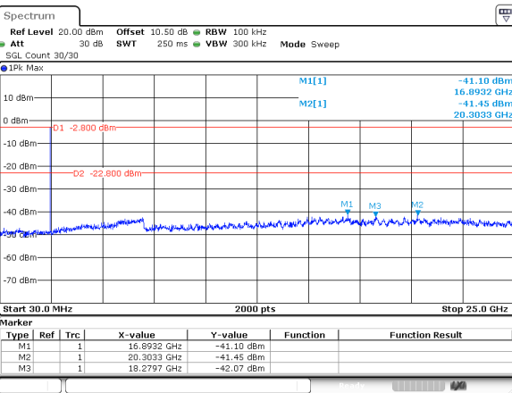
BLE_2M_High_Channel
