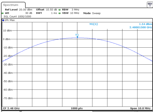
BLE_1M_High_Channel
