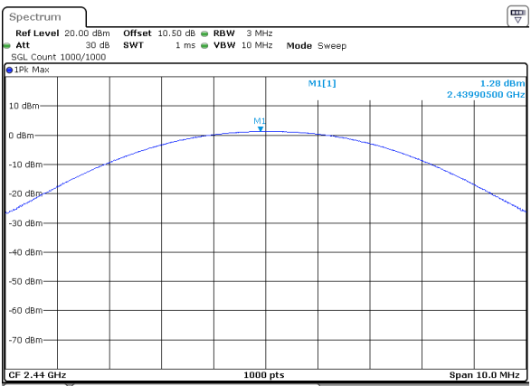
BLE_1M_Middle_Channel
