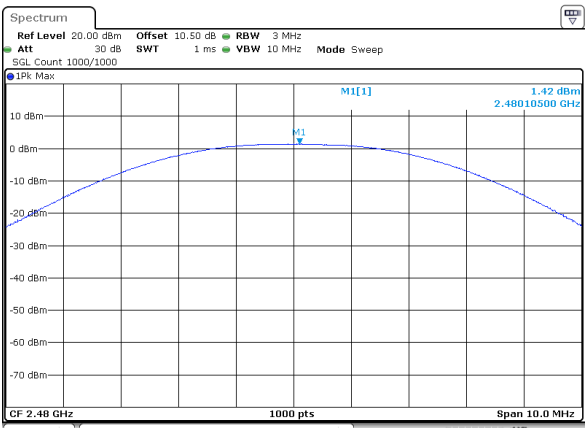
BLE_2M_High_Channel
