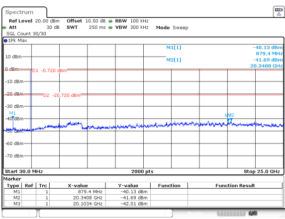
BLE_1M_Middle_Channel
