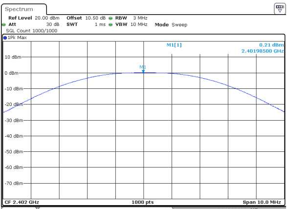
BLE_2M_Low_Channel
