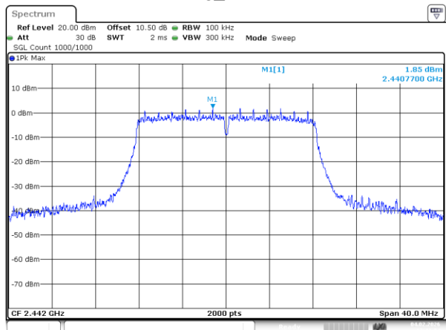
802.11g_2442MHz
