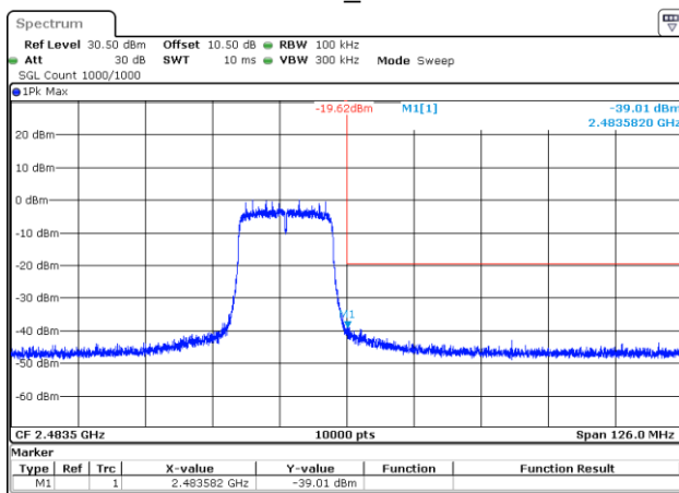
802.11n20_2472MHz
