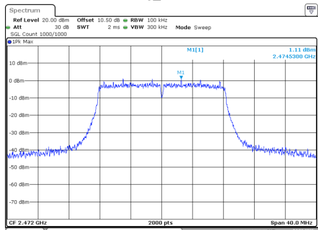
802.11g_2472MHz
