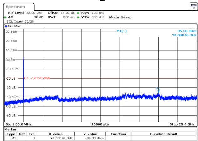
802.11n20_2472MHz
