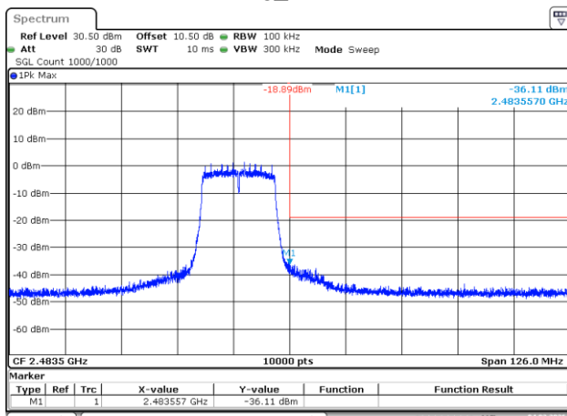
802.11g_2472MHz
