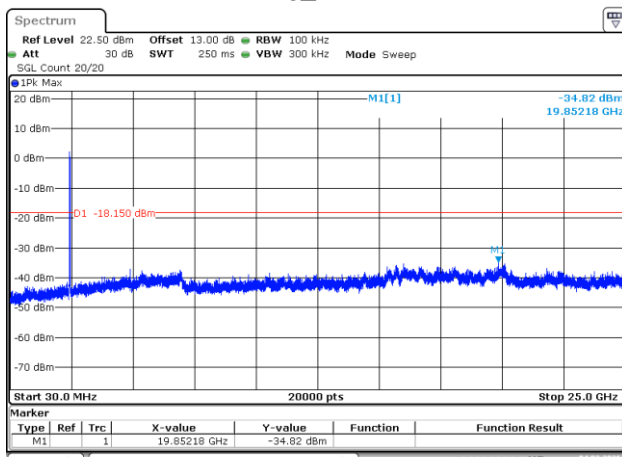
802.11g_2442MHz
