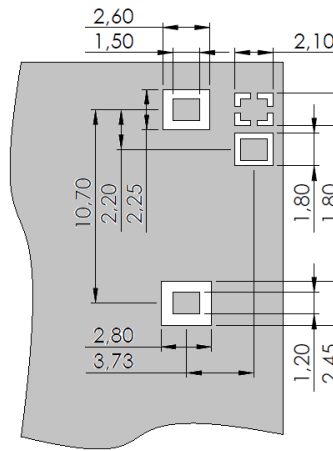
PCB Layout (from evaluation board)
