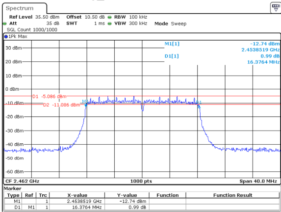
802.11g_2462MHz 16.376MHz
