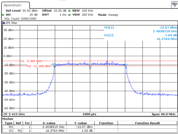
802.11g_2412MHz 16.376MHz
