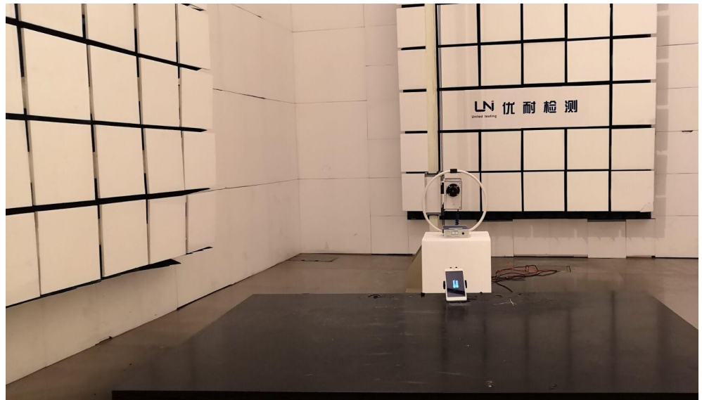
Radiated Emission (Below 30MHz)
