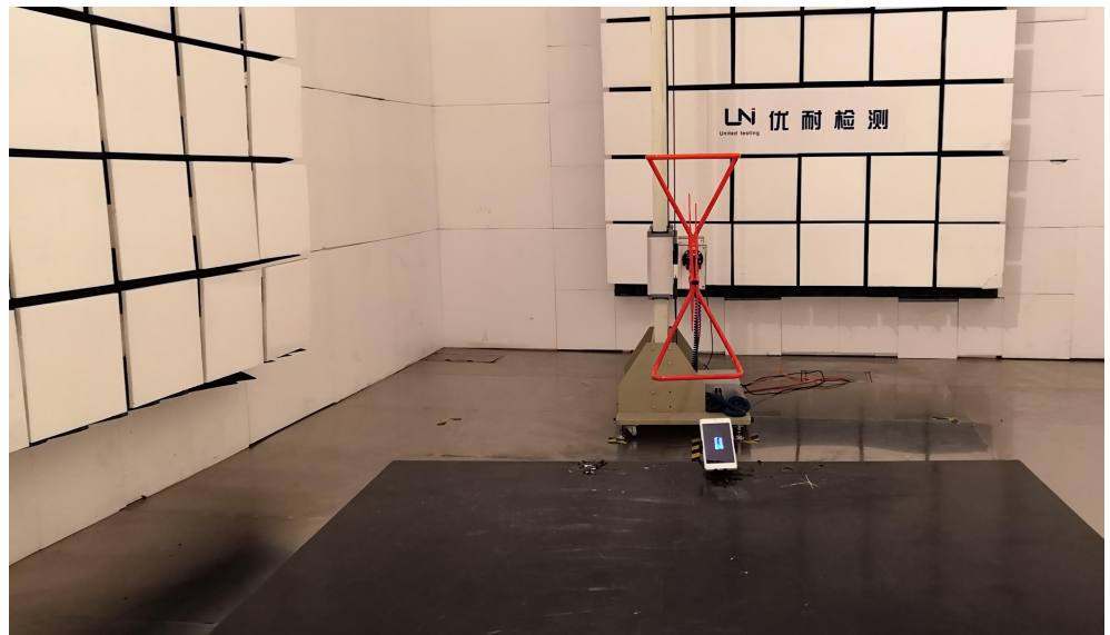
Radiated Emission (Below 1G)
