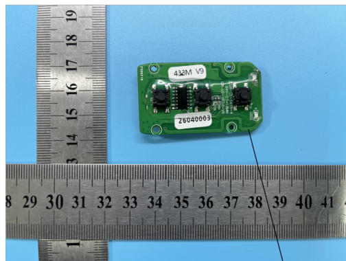
Antenna Location
