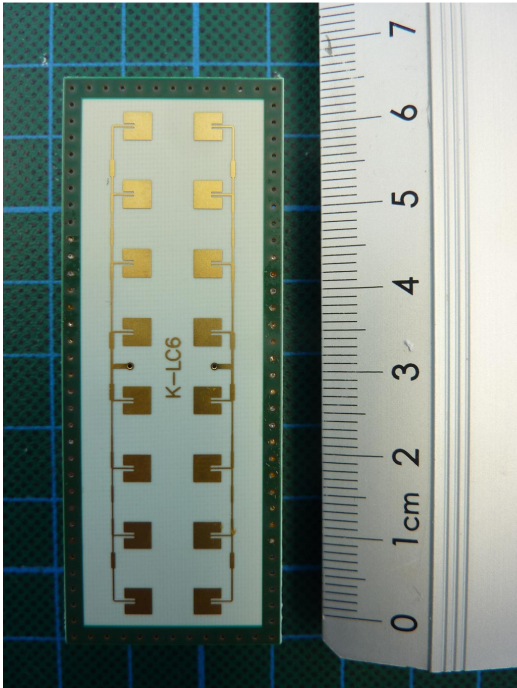
181709_a.jpg: K-LC6, front view
