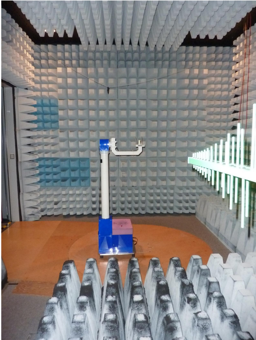
181709_13.jpg: K-LC6, test setup fully anechoic chamber
