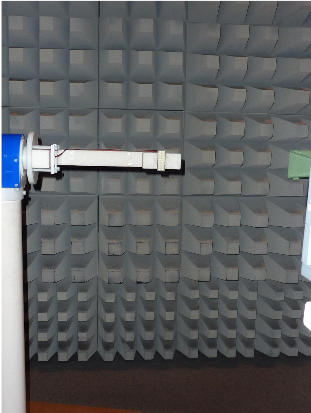
181709_15.jpg: K-LC6, test setup fully anechoic chamber
