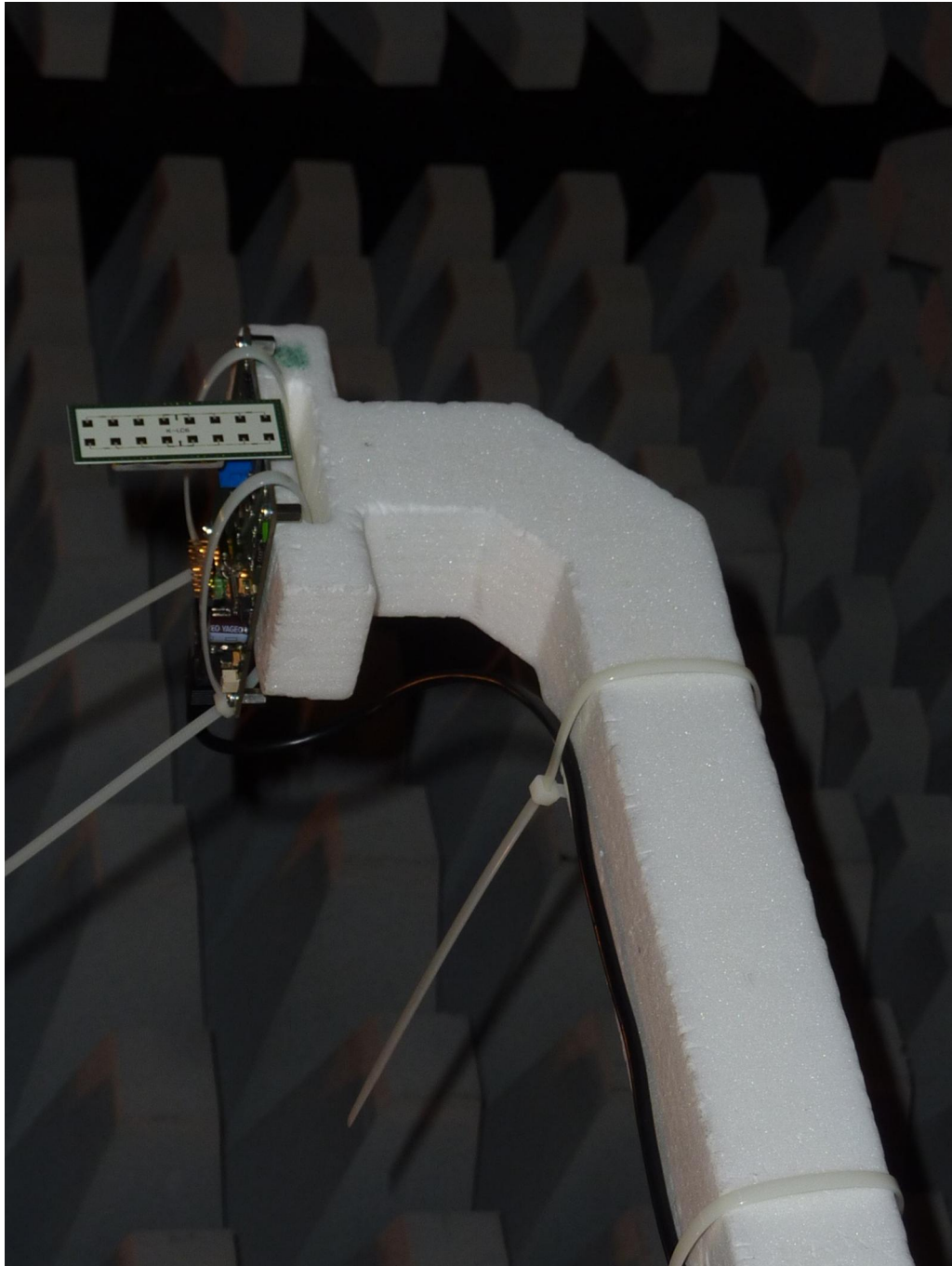
181709_11.jpg: K-LC6, test setup fully anechoic chamber
