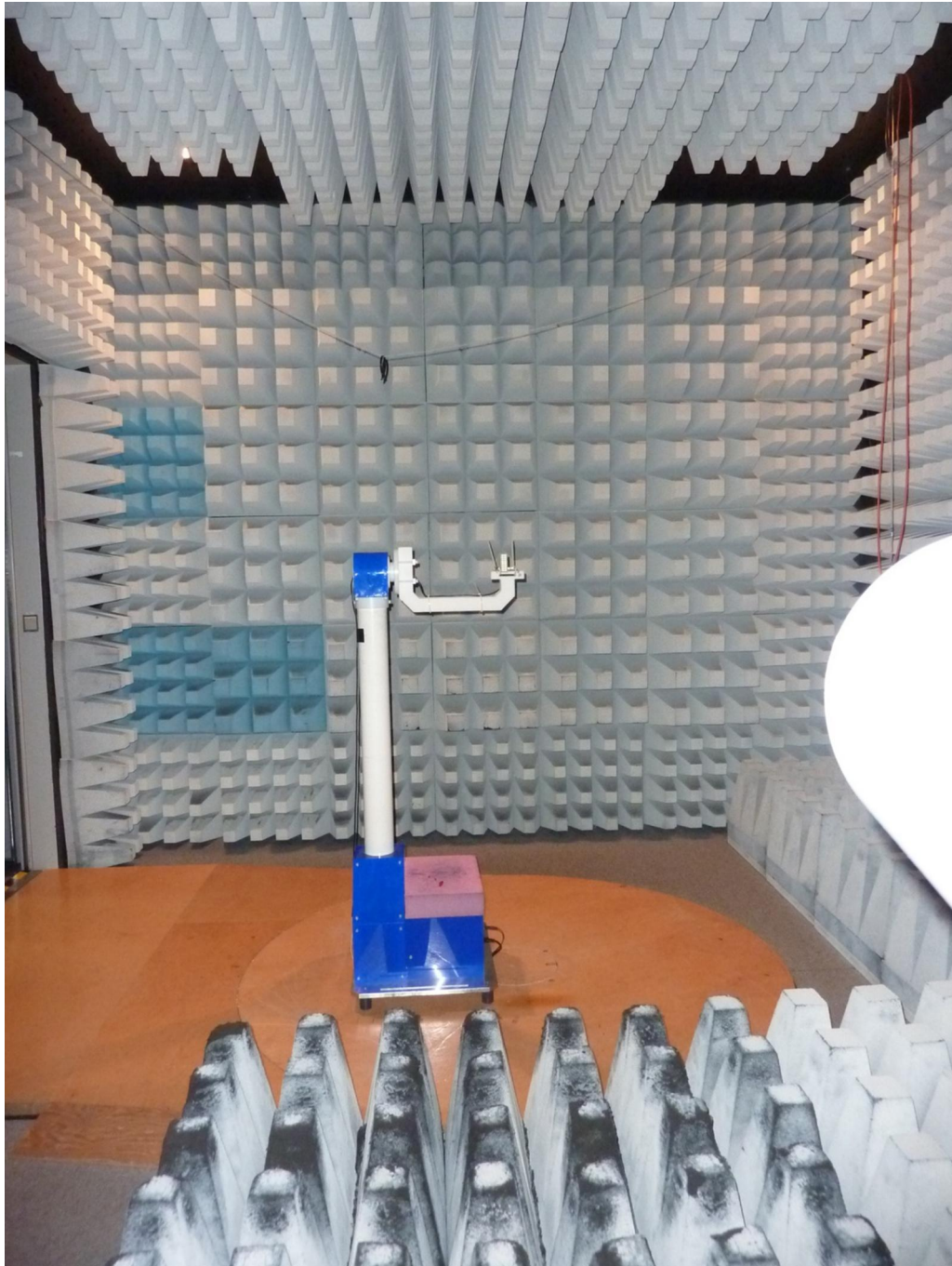
181709_14.jpg: K-LC6, test setup fully anechoic chamber
