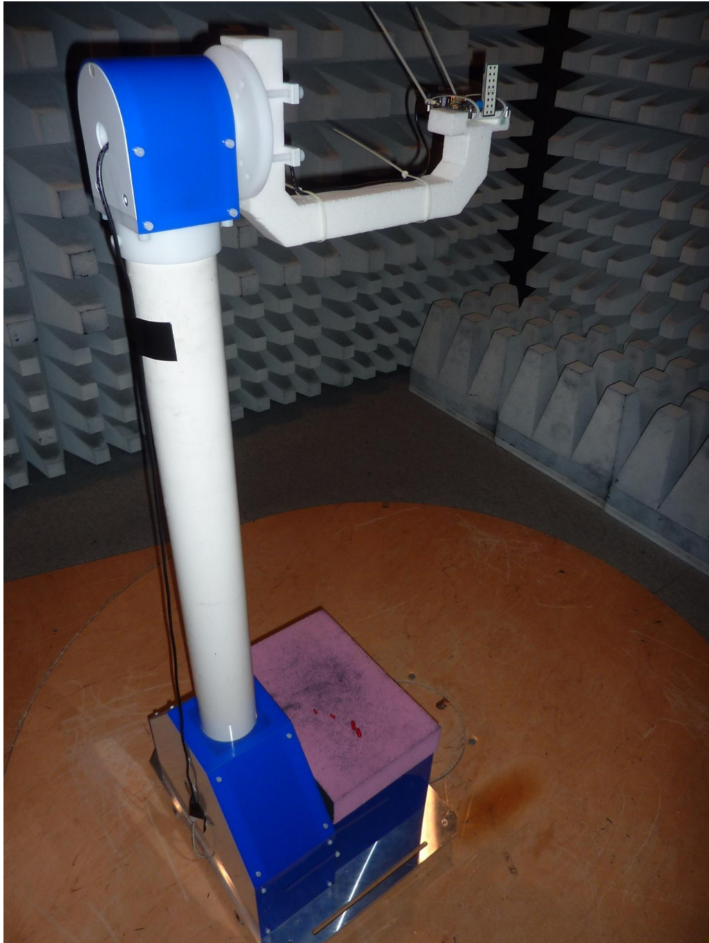
181709_10.jpg: K-LC6, test setup fully anechoic chamber
