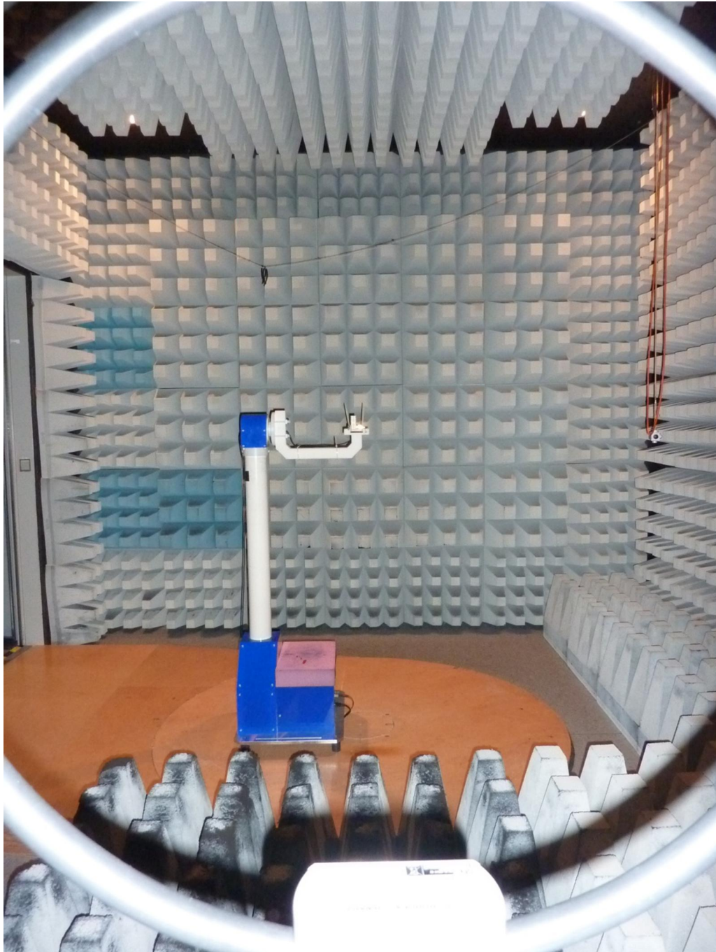
181709_12.jpg: K-LC6, test setup fully anechoic chamber
