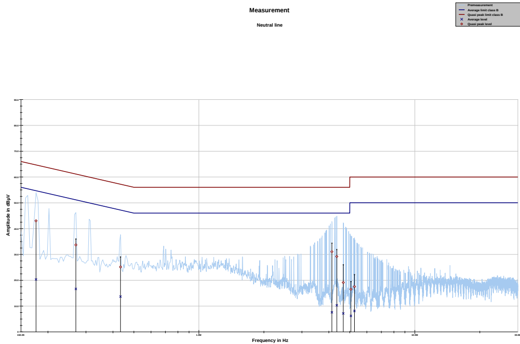
Plot 21: Neutral line
