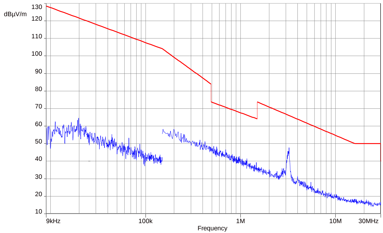
Plot No. 6: 9 kHz to 30 MHz, horizontal/vertical polarization, f_{\text{high}}
