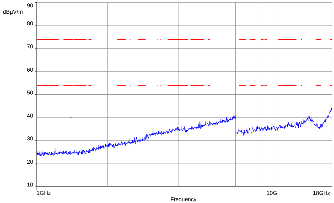
Plot No. 10: 1 GHz to 18 GHz, horizontal/vertical polarization, f_{\text{high}}
