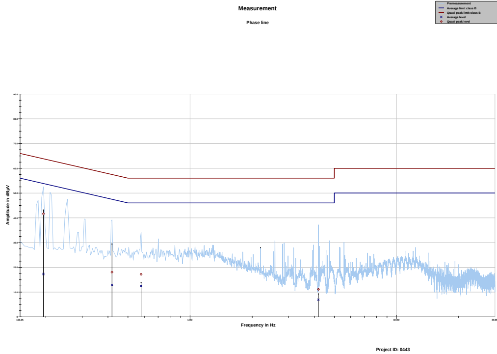
Plot 20: Phase line
