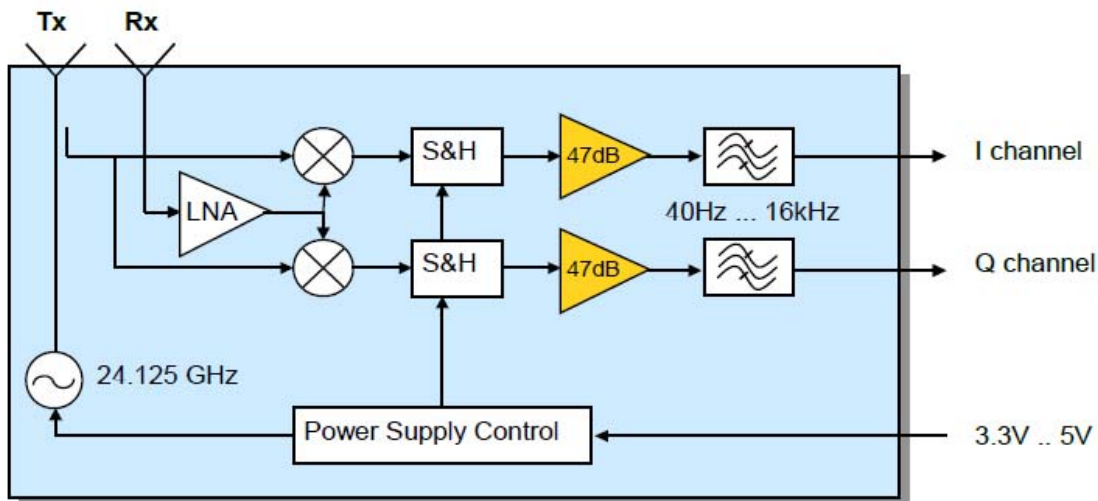
Fig. 1: K-MC1_LP Blockdiagram
