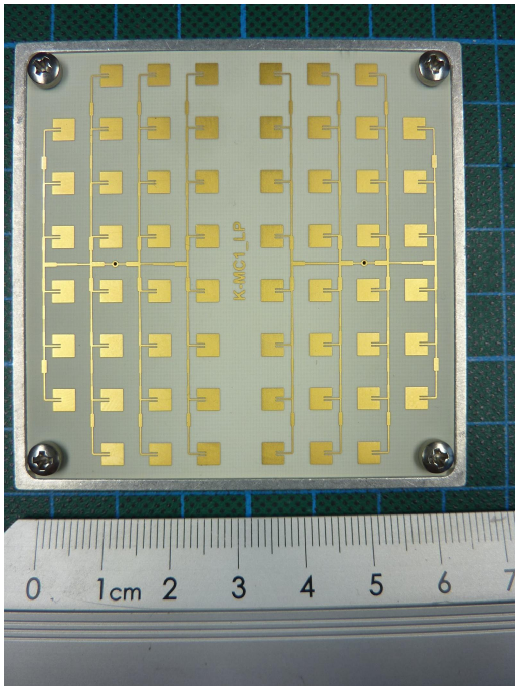
181708_g.jpg: K-MC1_LP, front view
