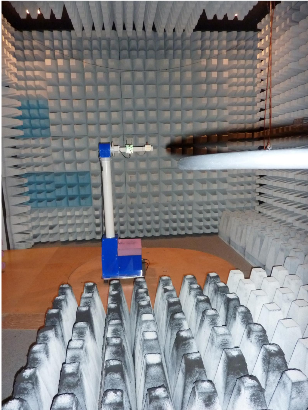
181708_11.jpg: K-MC1_LP, test setup fully anechoic chamber
