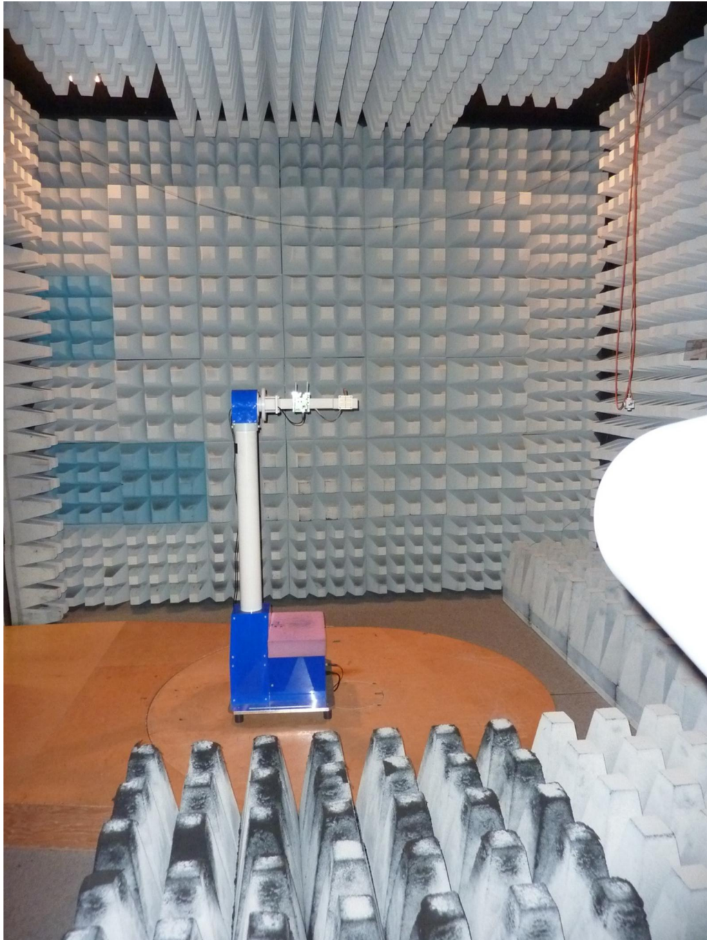
181708_13.jpg: K-MC1_LP, test setup fully anechoic chamber
