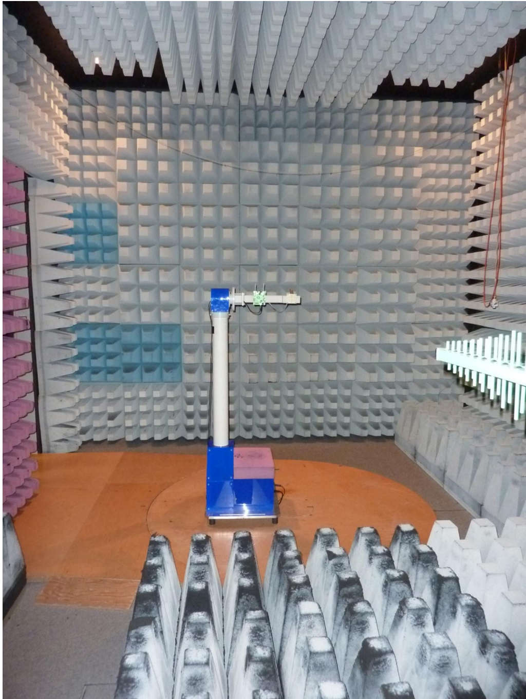
181708_12.jpg: K-MC1_LP, test setup fully anechoic chamber
