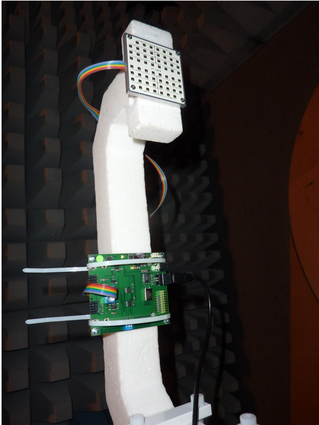
181708_10.jpg: K-MC1_LP, test setup fully anechoic chamber
