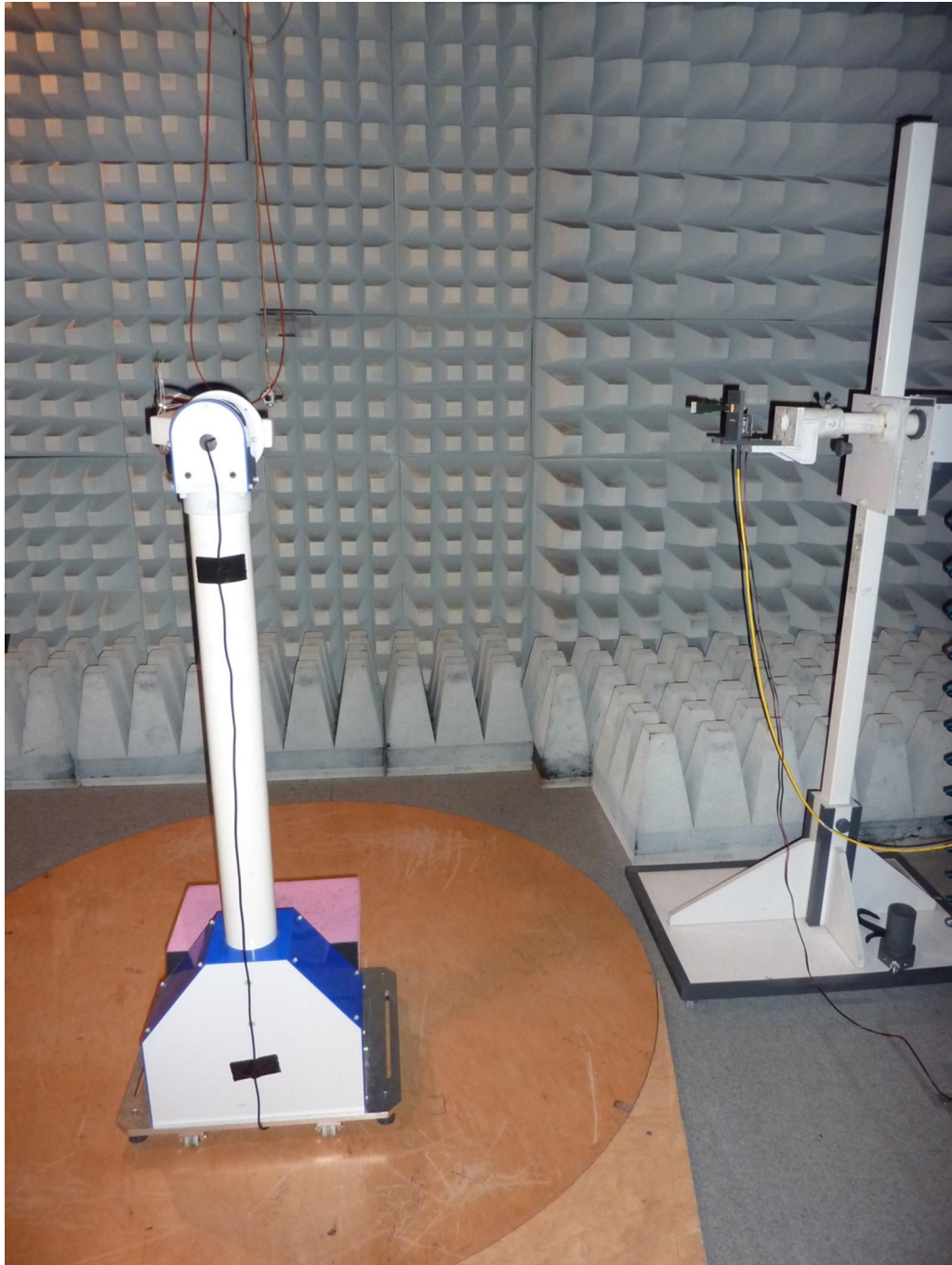
181708_14.jpg: K-MC1_LP, test setup fully anechoic chamber
