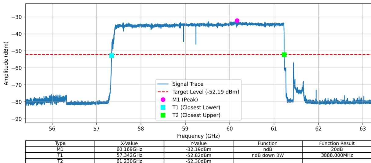
Plot: Peak power without lens
