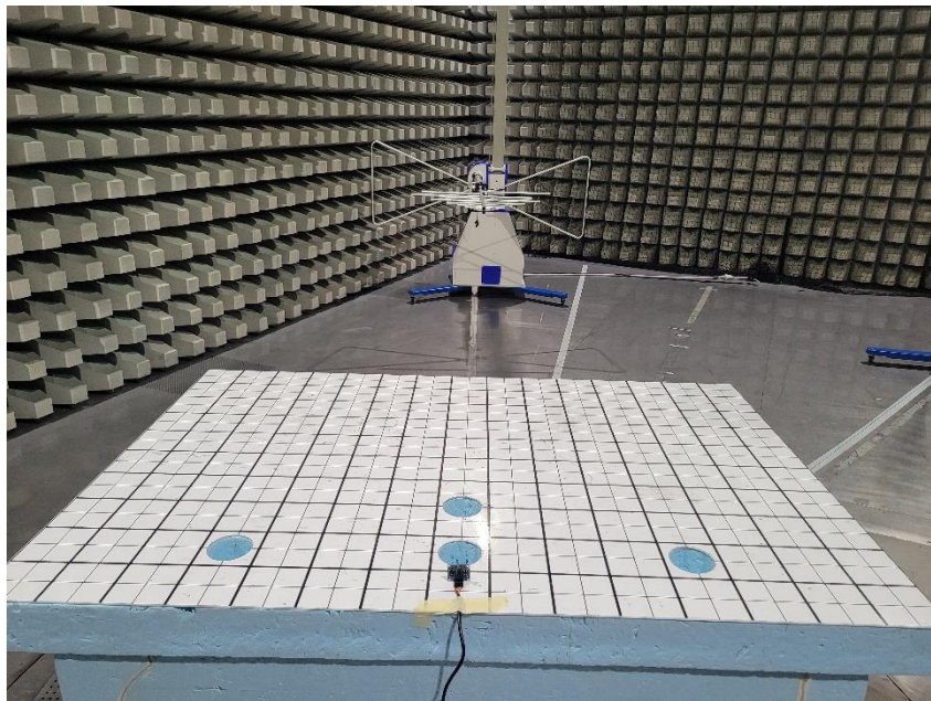
Photo 4 Radiated Test Setup from 30 MHz to 1 GHz
