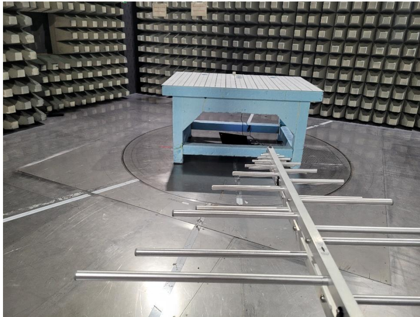
Photo 3 Radiated Test Setup from 30 MHz to 1 GHz
