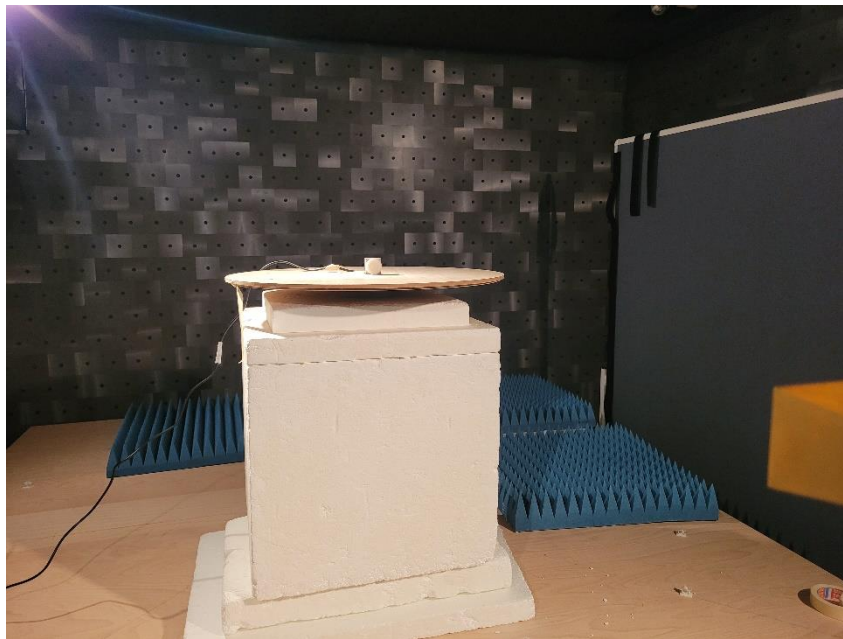
Photo 9 Radiated Test Setup above 40 GHz
