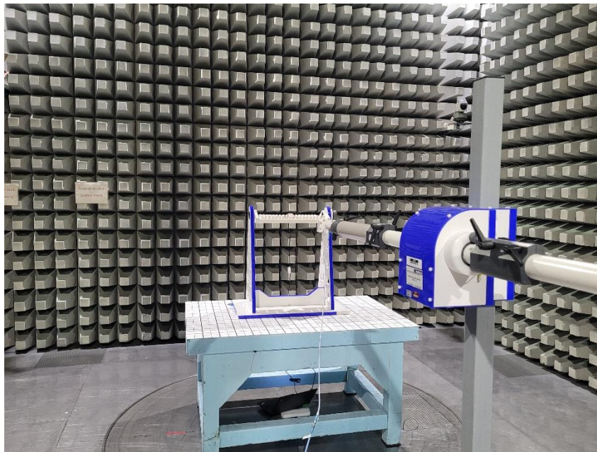
Photo 7 Radiated Test Setup 18-40 GHz
