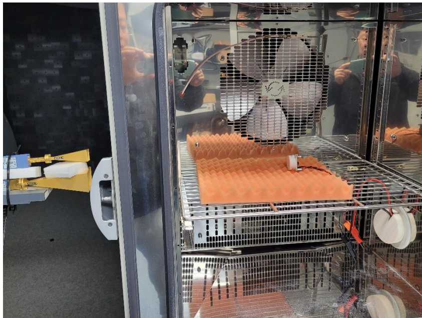
Photo 11 Test Setup frequency stability
