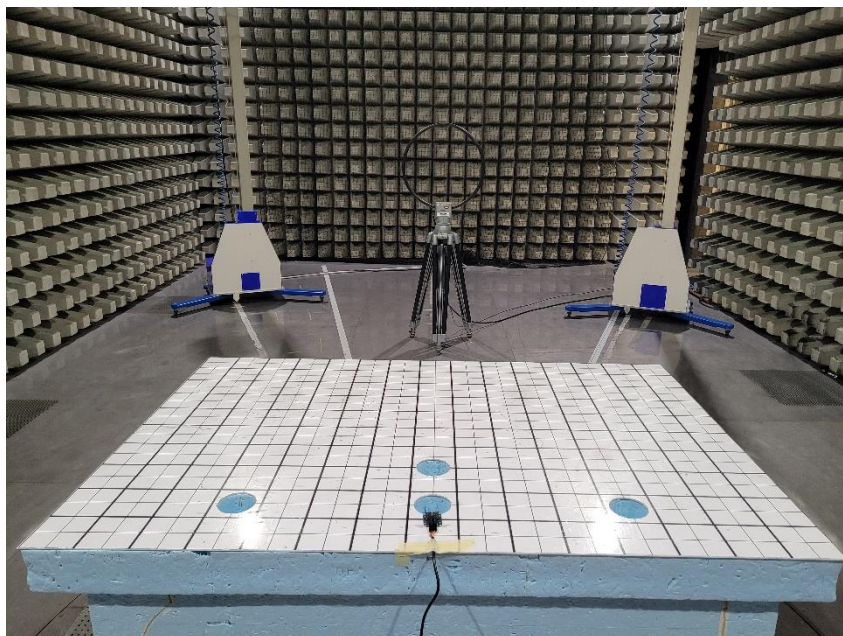
Photo 2 Radiated Test Setup below 30 MHz
