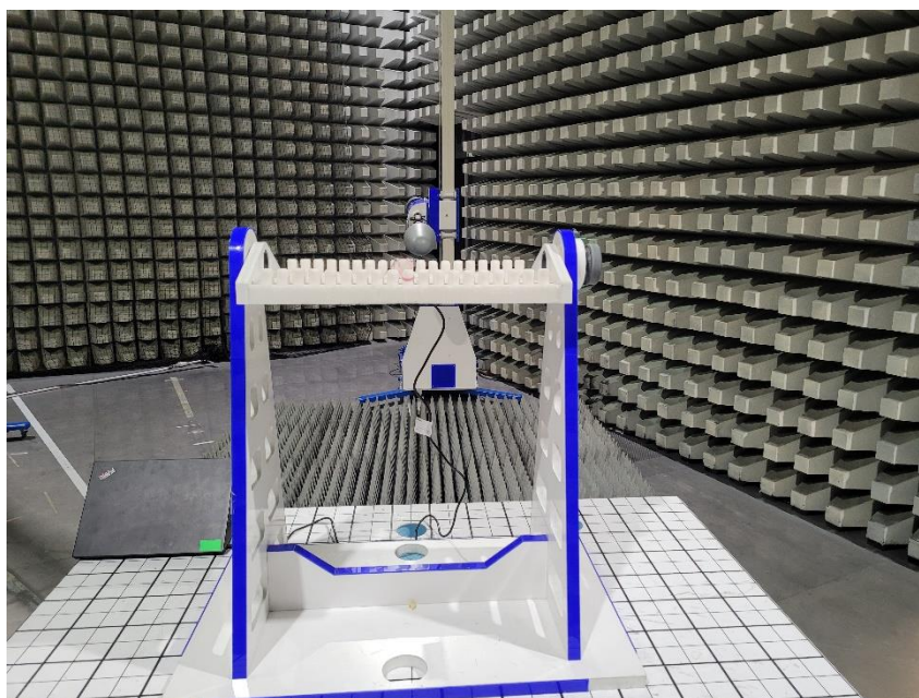
Photo 6 Radiated Test Setup 1 - 18 GHz
