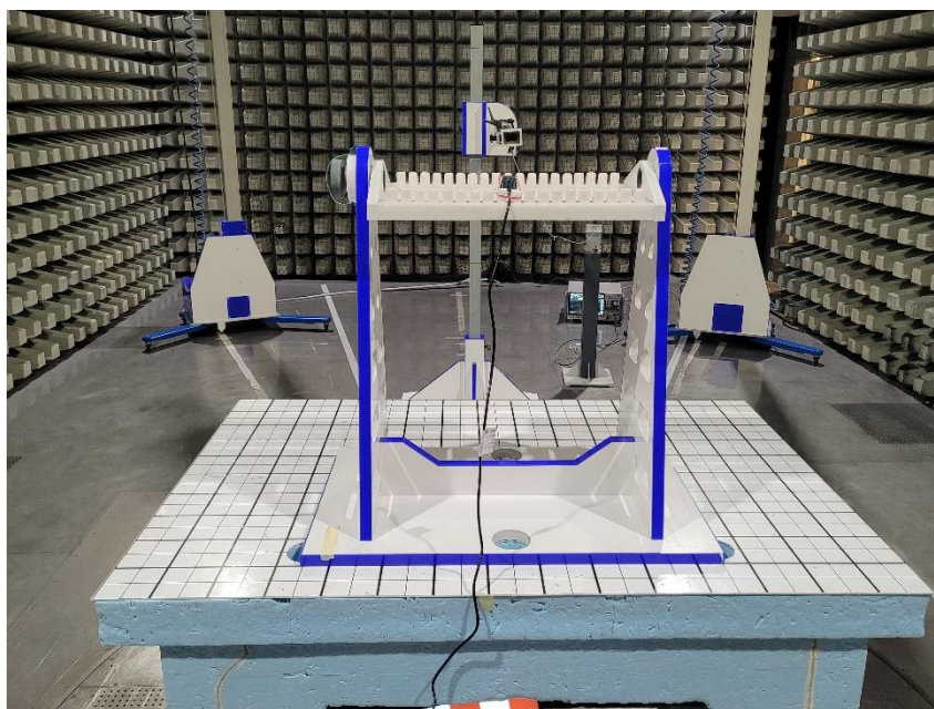
Photo 8 Radiated Test Setup 18-40 GHz
