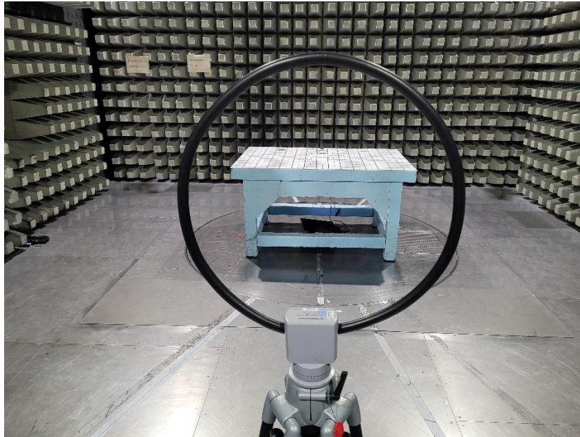
Photo 1 Radiated Test Setup below 30 MHz
