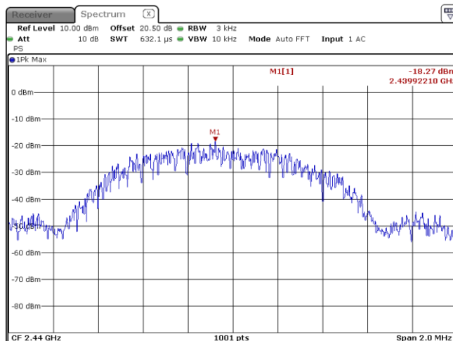
Figure 8.7-2: PSD for mid channel
