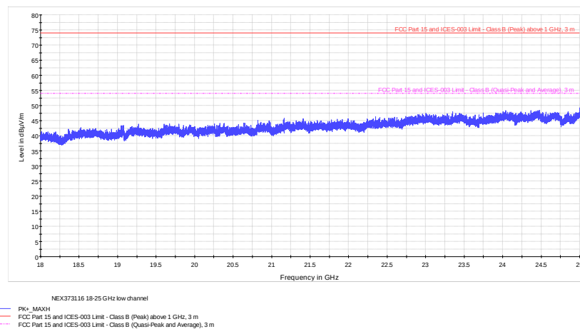
Figure 8.6-7: Radiated spurious emissions low channel 18-25 GHz
