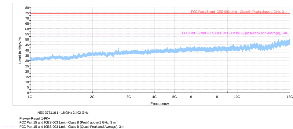
Figure 8.6-6: Radiated spurious emissions low channel 1-18 GHz
