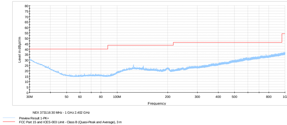
Figure 8.6-5: Radiated spurious emissions low channel 30-1000 MHz
