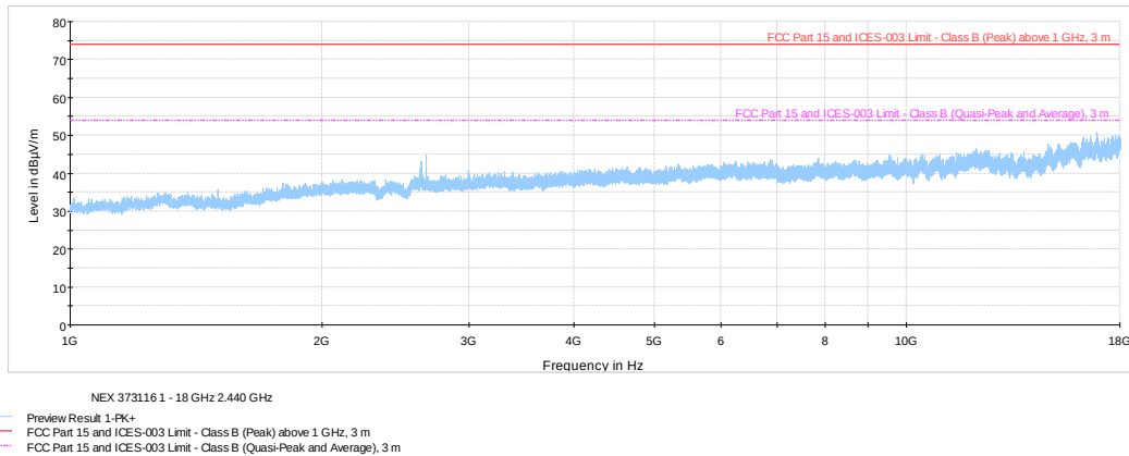
Figure 8.6-9: Radiated spurious emissions mid channel 1-18 GHz
