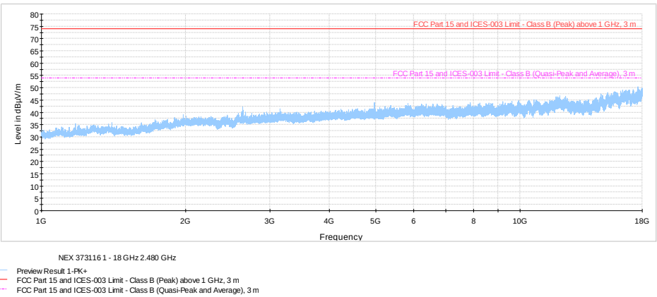
Figure 8.6-12: Radiated spurious emissions high channel 1-18 GHz
