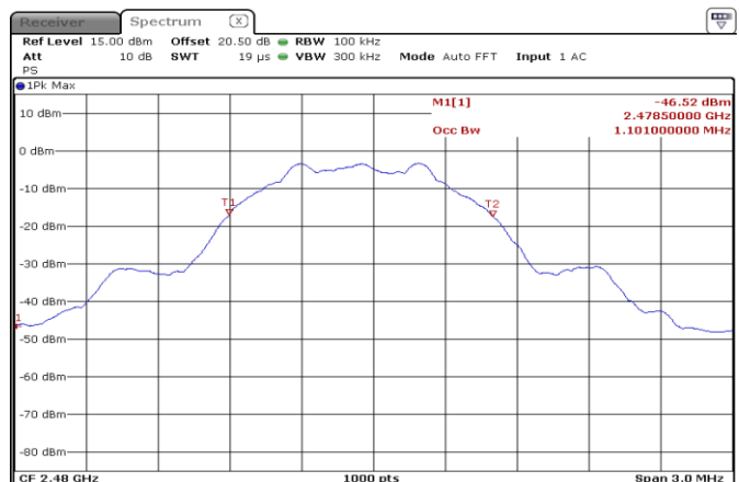
Figure 8.4-6: 99% occupied bandwidth on high channel
