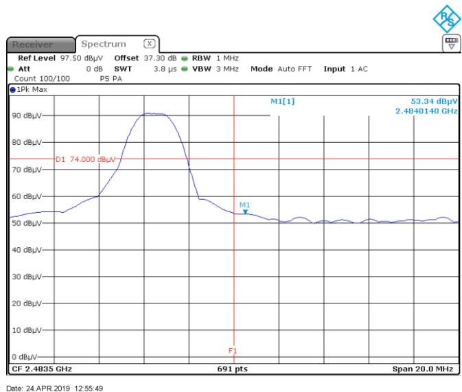
Figure 8.6-2: Radiated restricted upper band edge - Peak
