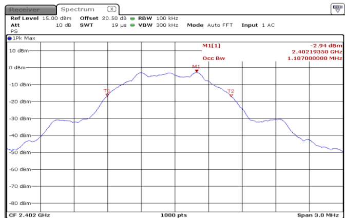
Figure 8.4-4: 99% occupied bandwidth on low channel
