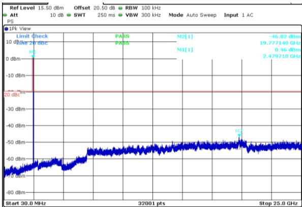
Figure 8.6-15: Conducted spurious emissions high channel
