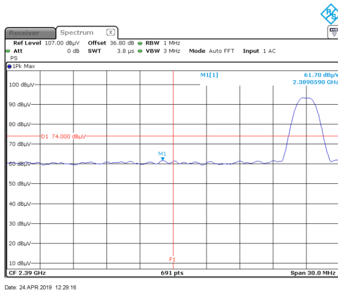
Figure 8.6-1: Radiated restricted lower band edge - Peak
