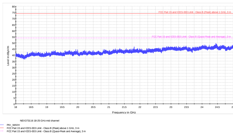
Figure 8.6-10: Radiated spurious emissions mid channel 18-25 GHz
