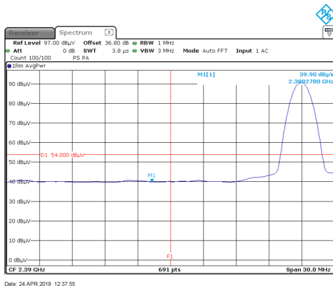
Figure 8.6-3: Radiated restricted lower band edge - Average
