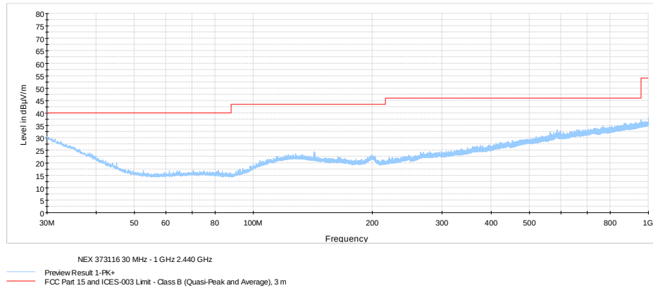
Figure 8.6-8: Radiated spurious emissions mid channel 30-1000 MHz
