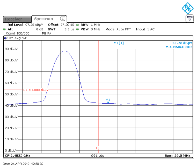
Figure 8.6-4: Radiated restricted upper band edge - Average
