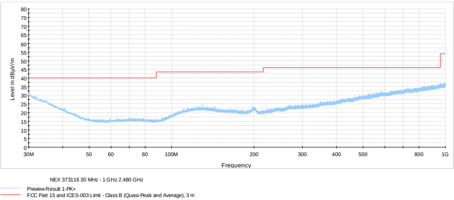
Figure 8.6-11: Radiated spurious emissions high channel 30-1000 MHz
