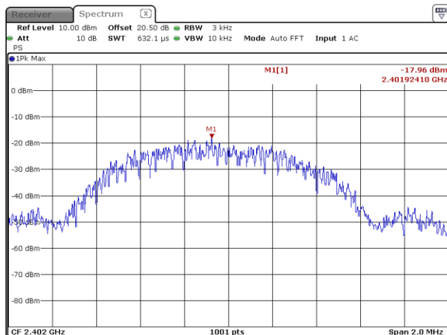
Figure 8.7-1: PSD for low channel
