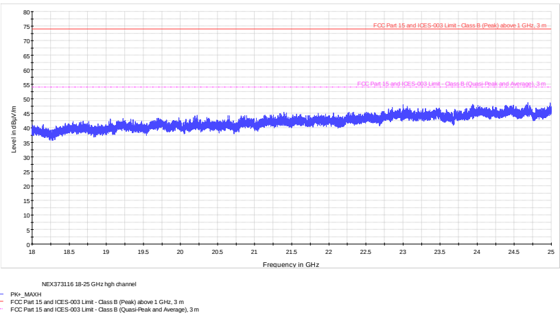
Figure 8.6-13: Radiated spurious emissions high channel 18-25 GHz
