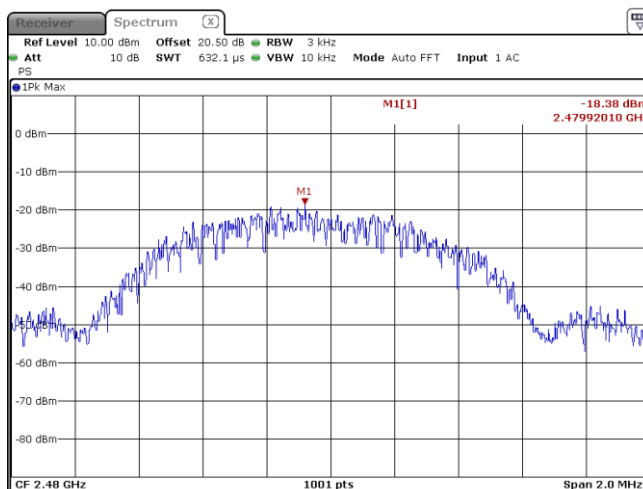
Figure 8.7-3: PSD for high channel
