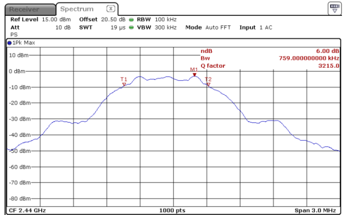
Figure 8.4-2: 6 dB bandwidth on mid channel
