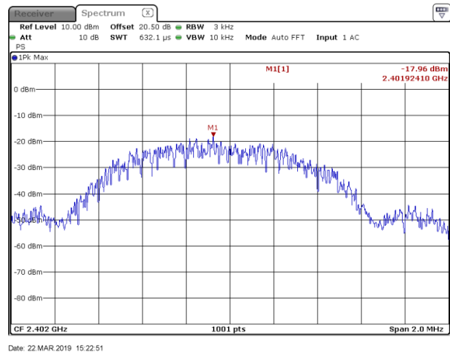
Figure 8.7-1: PSD for low channel
