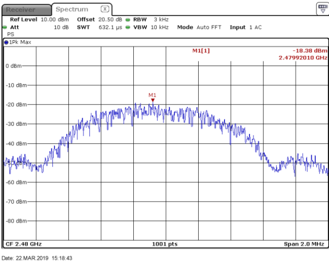
Figure 8.7-3: PSD for high channel
