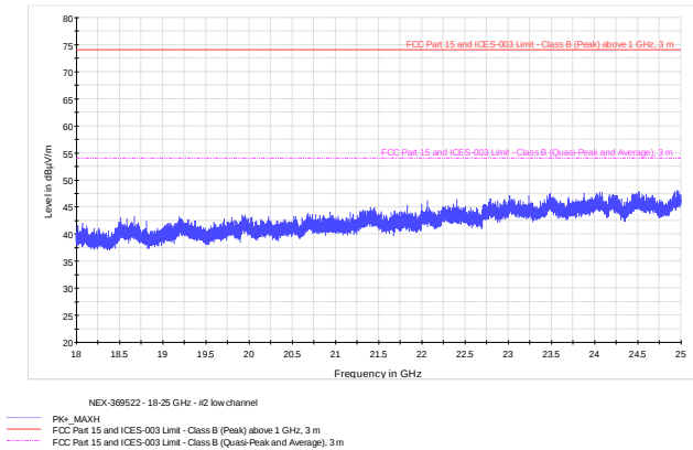
Figure 8.6-7: Radiated spurious emissions low channel 18-25 GHz
