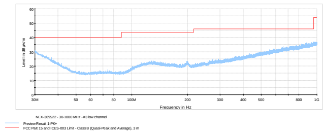
Figure 8.6-5: Radiated spurious emissions low channel 30-1000 MHz
