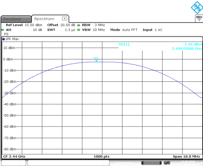
Figure 8.5-2: Output power on mid channel
