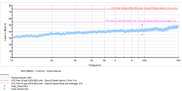
Figure 8.6-6: Radiated spurious emissions low channel 1-18 GHz
