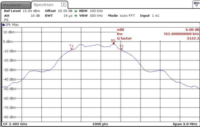
Figure 8.4-1: 6 dB bandwidth on low channel
