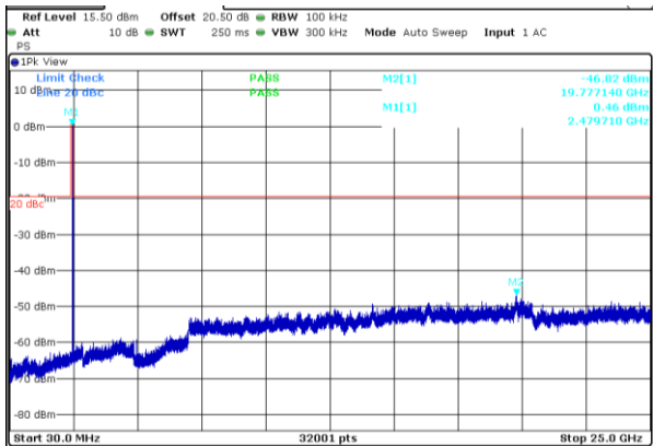
Figure 8.6-15: Conducted spurious emissions high channel
