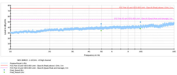
Figure 8.6-12: Radiated spurious emissions high channel 1-18 GHz
