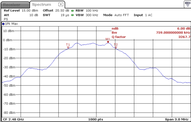
Figure 8.4-3: 6 dB bandwidth on high channel
