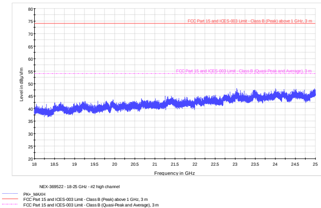
Figure 8.6-13: Radiated spurious emissions high channel 18-25 GHz
