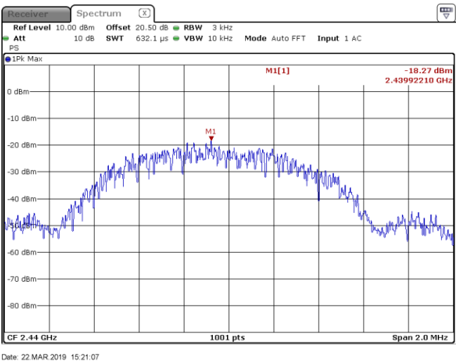
Figure 8.7-2: PSD for mid channel
