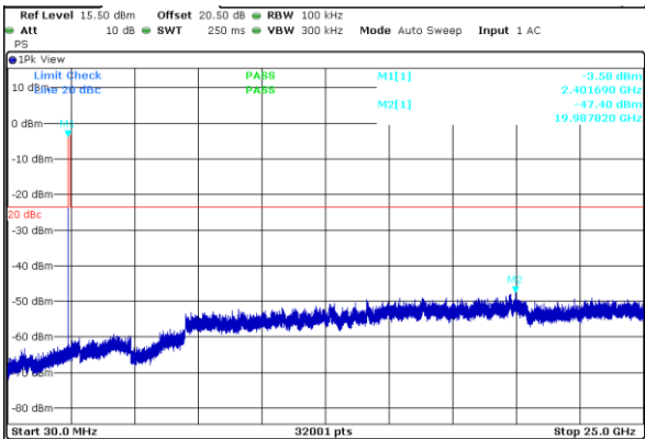
Figure 8.6-14: Conducted spurious emissions low channel
