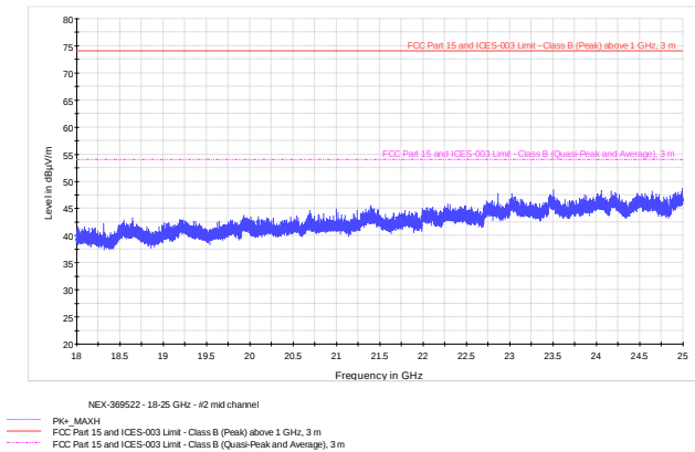
Figure 8.6-10: Radiated spurious emissions mid channel 18-25 GHz
