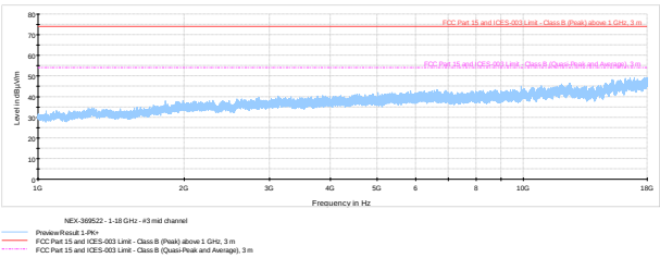
Figure 8.6-9: Radiated spurious emissions mid channel 1-18 GHz
