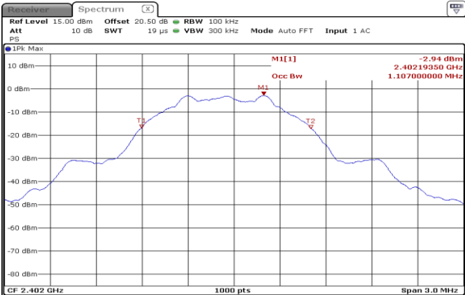
Figure 8.4-4: 99% occupied bandwidth on low channel
