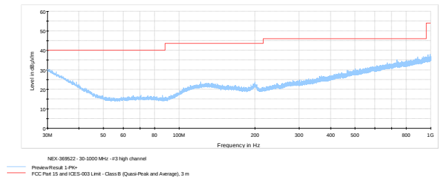
Figure 8.6-11: Radiated spurious emissions high channel 30-1000 MHz
