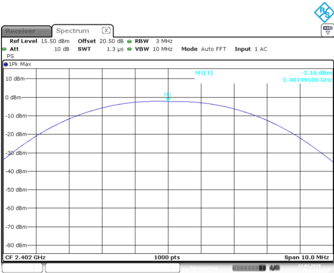
Figure 8.5-1: Output power on low channel
