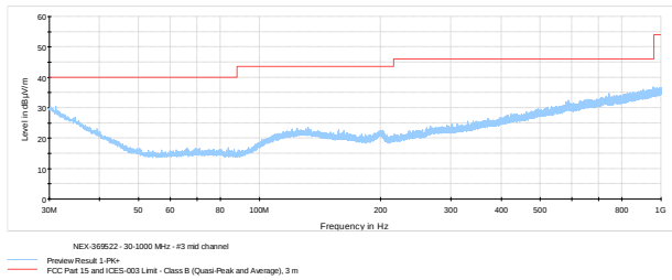
Figure 8.6-8: Radiated spurious emissions mid channel 30-1000 MHz
