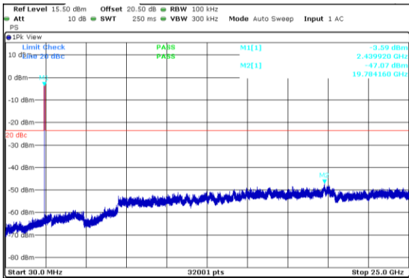
Figure 8.6-15: Conducted spurious emissions mid channel
