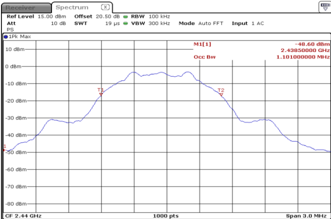
Figure 8.4-5: 99% occupied bandwidth on mid channel
