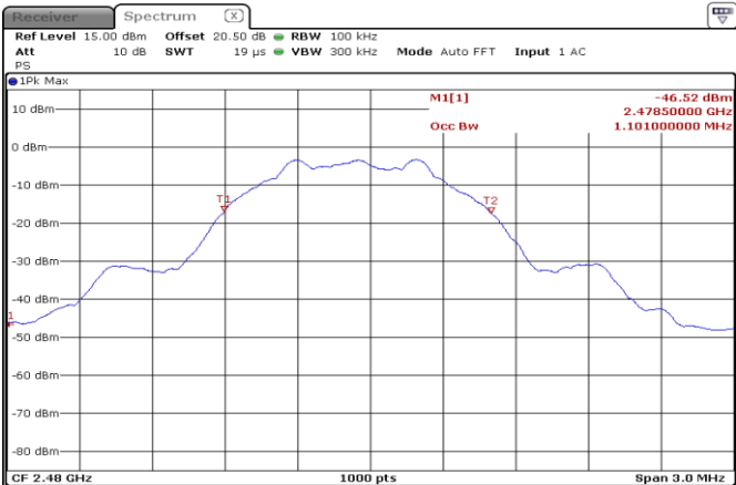
Figure 8.4-6: 99% occupied bandwidth on high channel
