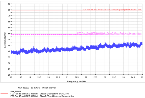
Figure 8.6-13: Radiated spurious emissions high channel 18-25 GHz
