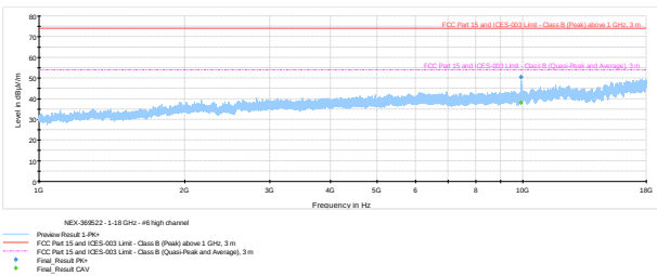
Figure 8.6-12: Radiated spurious emissions high channel 1-18 GHz
