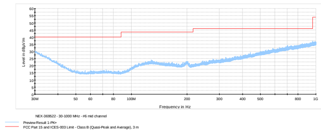
Figure 8.6-8: Radiated spurious emissions mid channel 30-1000 MHz
