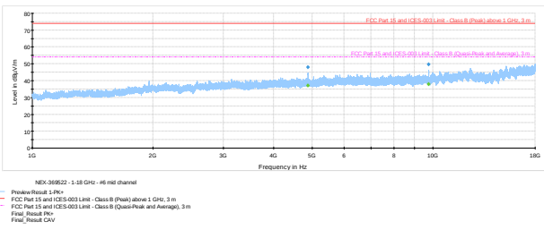
Figure 8.6-9: Radiated spurious emissions mid channel 1-18 GHz
