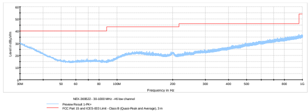
Figure 8.6-5: Radiated spurious emissions low channel 30-1000 MHz
