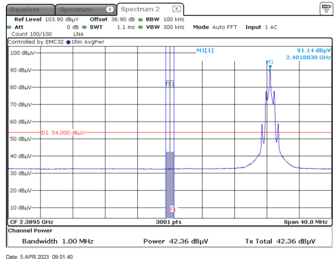
Figure 8.6-2: Band edge spurious emissions at 2390 MHz, Average, 1MHz
