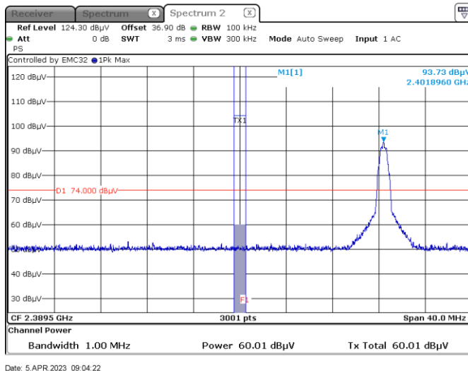
Figure 8.6-1: Band edge spurious emissions at 2390 MHz, Peak, 1MHz
