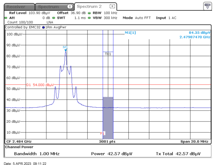
Figure 8.6-4: Band edge spurious emissions at 2483.5 MHz, Average, 1MHz
