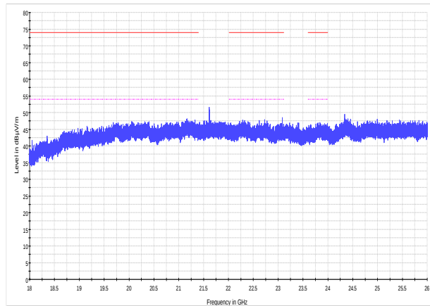
PRJ0024813 RE Spurious 18-26 GHz Low channel PK+ MAOH FCC 15.209 and RSS-Gen Restricted bands peak limits FCC 15.209 and RSS-Gen Restricted bands average limits
