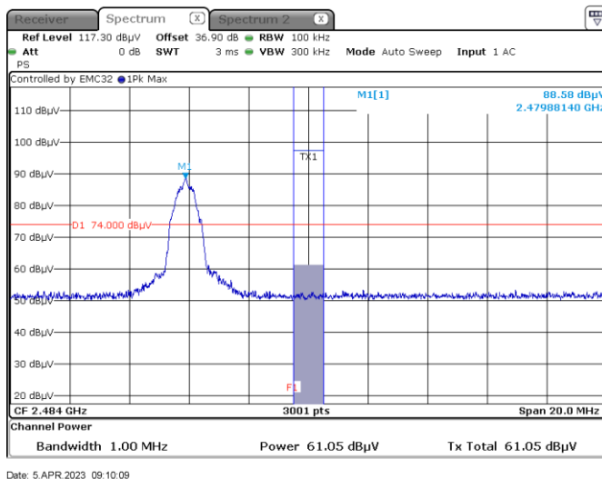
Figure 8.6-3: Band edge spurious emissions at 2483.5 MHz, Peak, 1MHz
