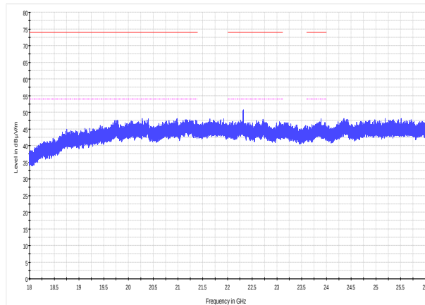
PRJ0024813 RE Spurious 18-26 GHz High channel PK+ MAOH FCC 15.209 and RSS-Gen Restricted bands peak limits FCC 15.209 and RSS-Gen Restricted bands average limits
