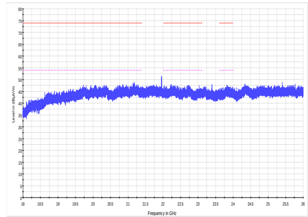
PRJ0024813 RE Spurious 18-26 GHz Mid channel PK+ MAOH FCC 15.209 and RSS-Gen Restricted bands peak limits FCC 15.209 and RSS-Gen Restricted bands average limits
