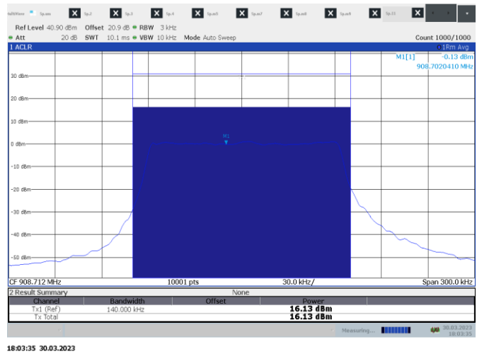
Figure 8.5-4: Output power on mid channel, 125 kHz BW
