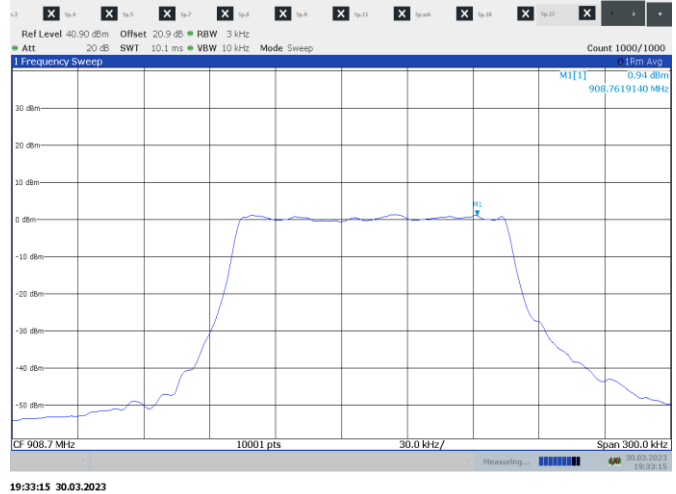
Figure 8.9-2: PSD on mid channel, 125 kHz BW
