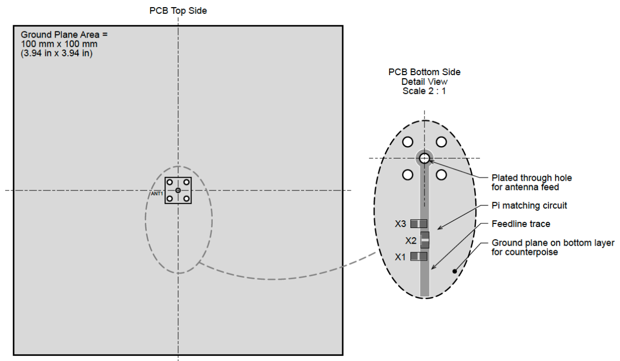
Figure 8. ANT-915-VHETH Recommended Layout
