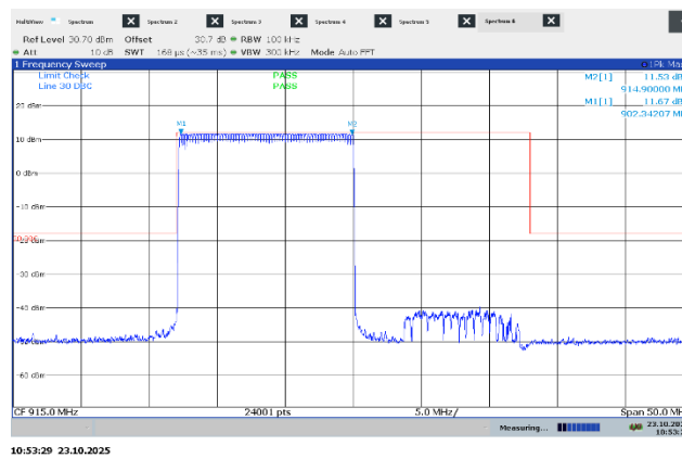
Figure 7.8-9: Conducted non-restricted band edge emissions, Hopping ON
