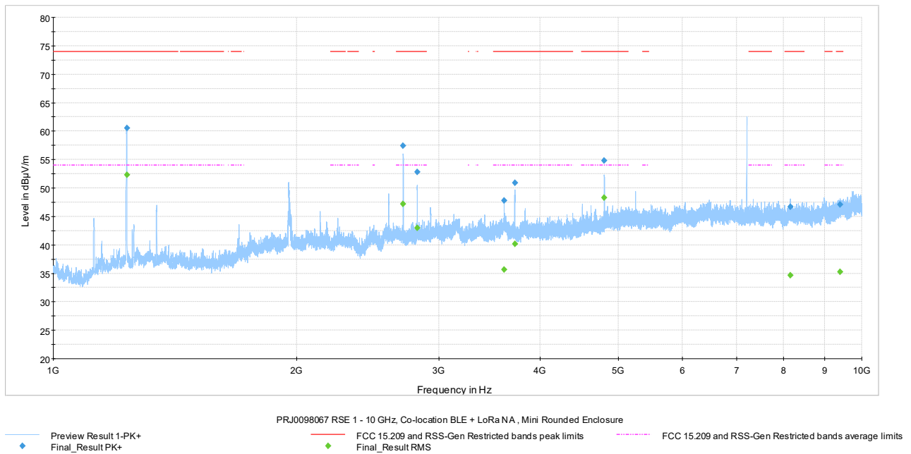
Figure 7.8-29: Radiated spurious emissions 1-10 GHz, 24/7 iQ TOTAL
