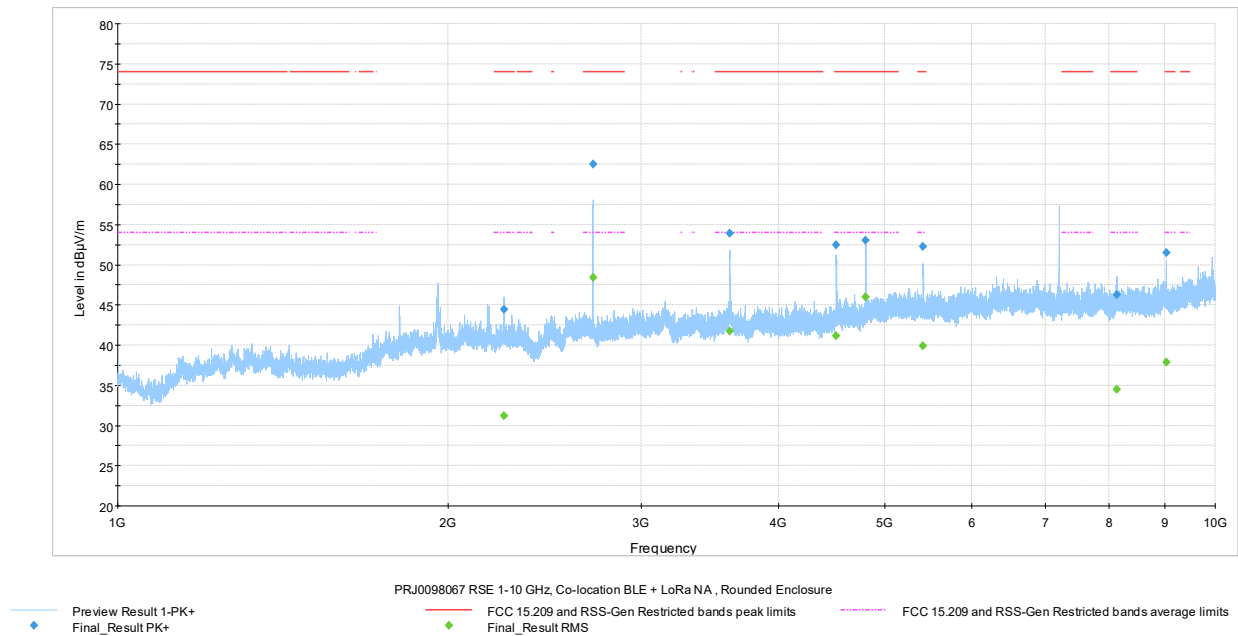
Figure 7.8-19: Radiated spurious emissions 1-10 GHz, Pulse Rat iQ TOTAL
