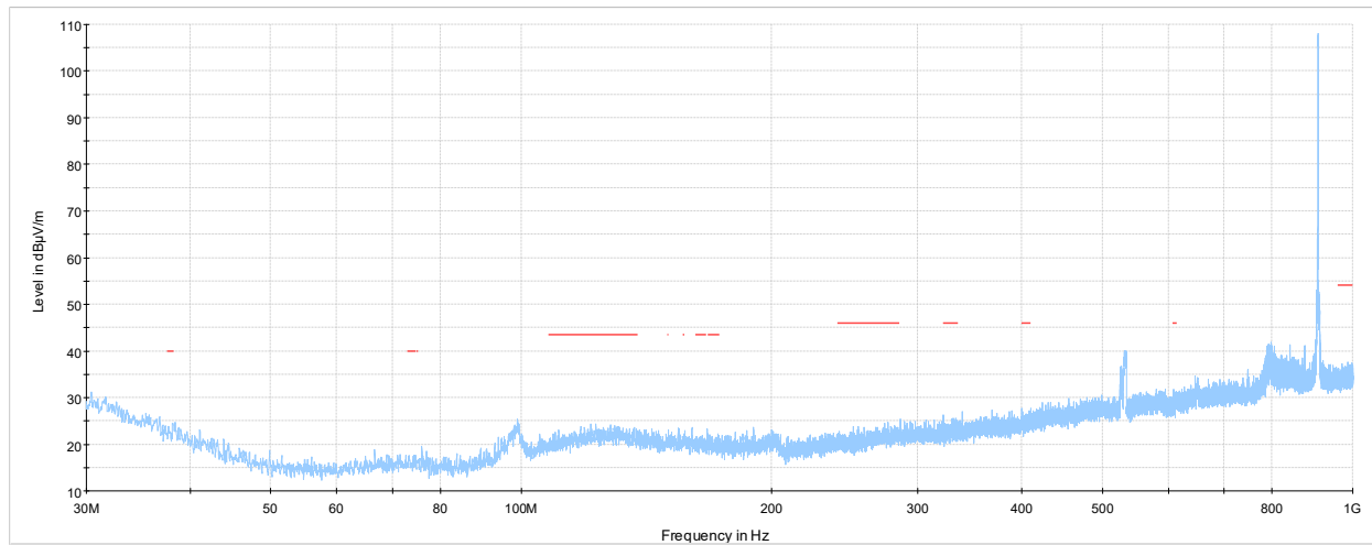
Figure 7.8-10: Radiated spurious emissions 30-1000 MHz low channel
