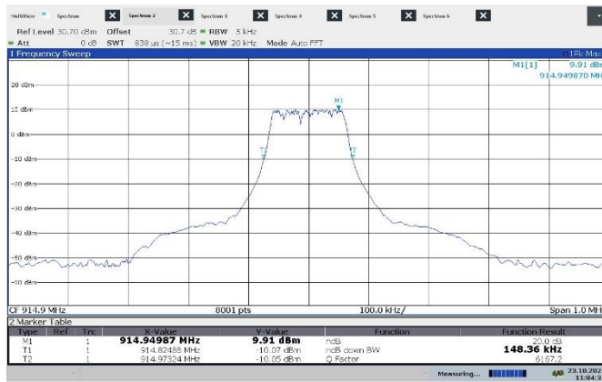
Figure 7.4-3: 20 dB bandwidth on high channel
