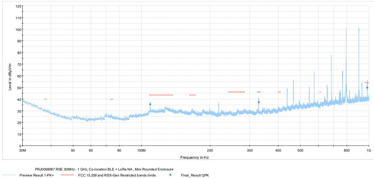
Figure 7.8-28: Radiated spurious emissions 30-1000 MHz, 24/7 iQ TOTAL
