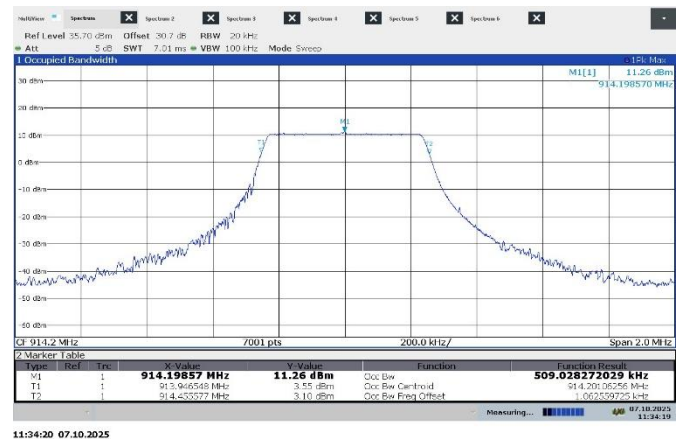
Figure 7.6-6: 99% occupied bandwidth on high ch, 500 kHz bandwidth signal
