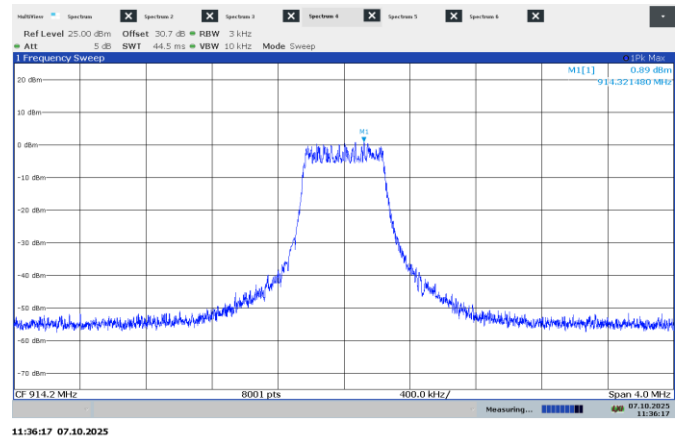
Figure 7.9-6: PSD on high channel, 500 kHz signal
