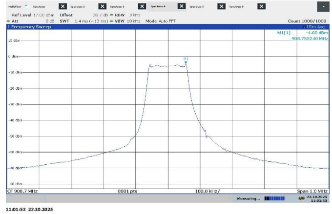
Figure 7.9-2: PSD on mid channel, 125 kHz signal
