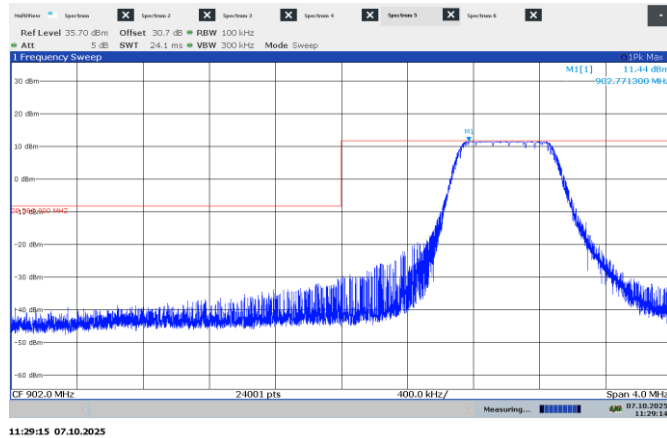
Figure 7.8-16: Conducted non-restricted band edge emissions at 902 MHz
