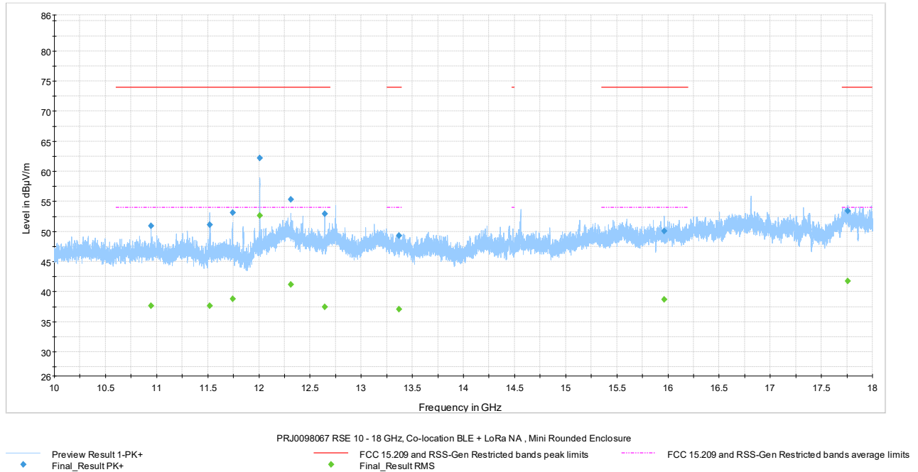
Figure 7.8-31: Radiated spurious emissions 10-18 GHz, 24/7 iQ TOTAL
