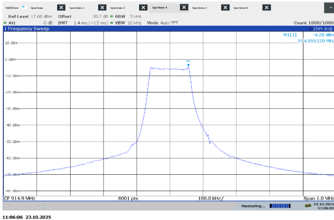
Figure 7.9-3: PSD on high channel, 125 kHz signal
