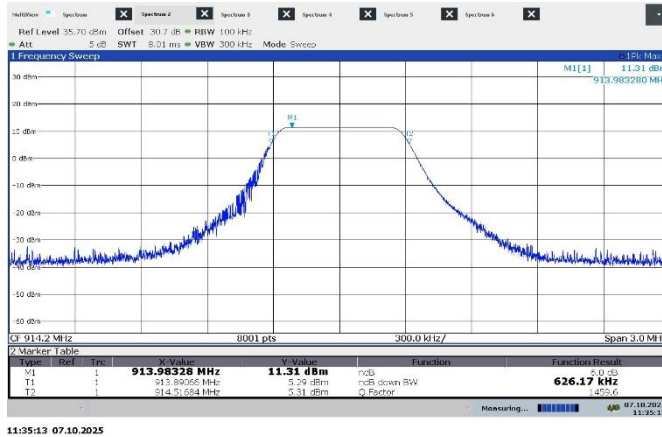
Figure 7.6-3: 6 dB bandwidth on high ch, 500 kHz bandwidth signal
