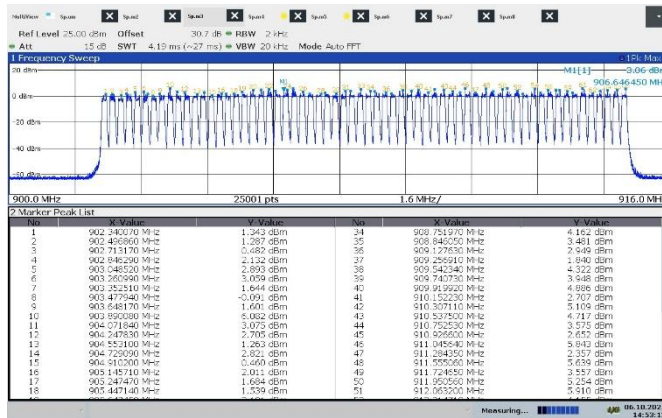
Figure 7.4-5: Number of hopping channels
