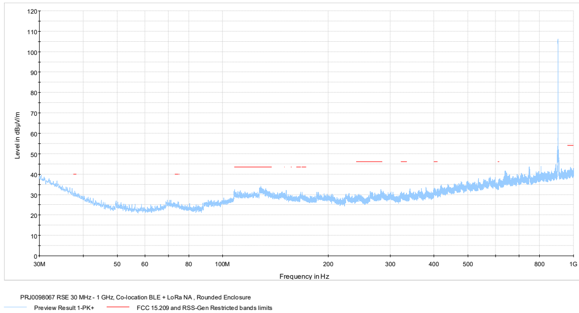
Figure 7.8-18: Radiated spurious emissions 30-1000 MHz, Pulse Rat iQ TOTAL
