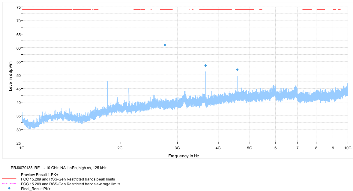
Figure 7.8-6: Radiated spurious emissions 1-10 GHz high channel
