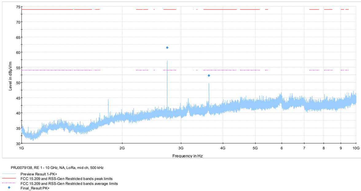
Figure 7.8-14: Radiated spurious emissions 1-10 GHz mid channel
