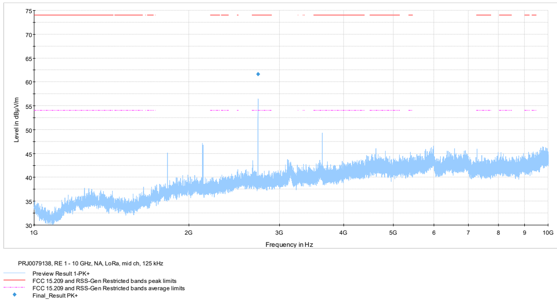
Figure 7.8-5: Radiated spurious emissions 1-10 GHz mid channel
