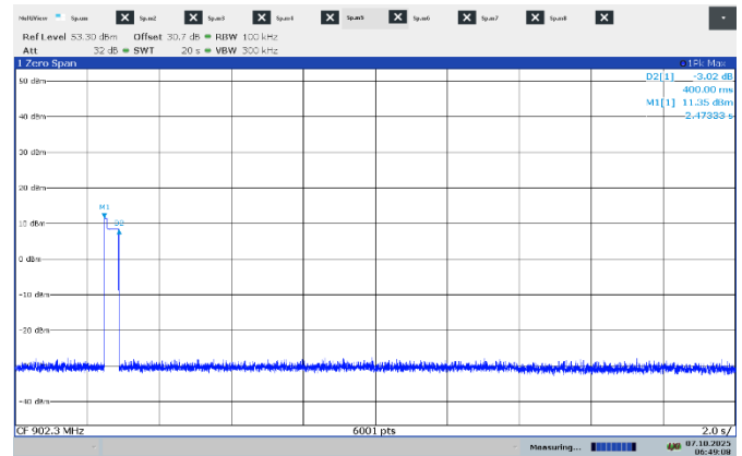
Figure 7.4-6: Dwell time
