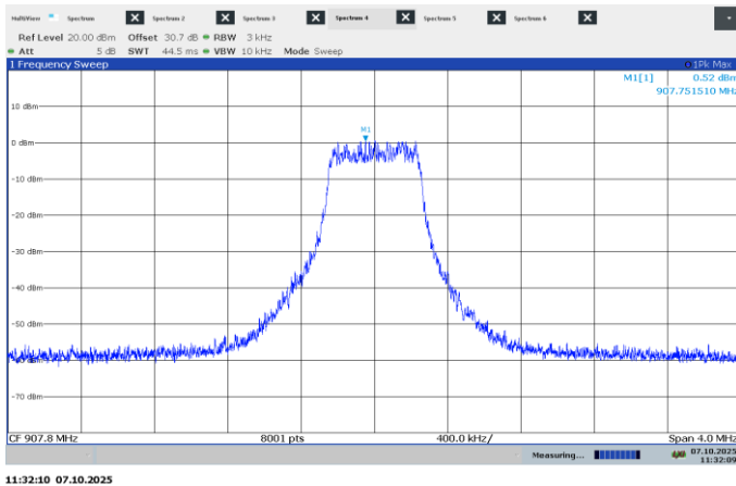
Figure 7.9-5: PSD on mid channel, 500 kHz signal
