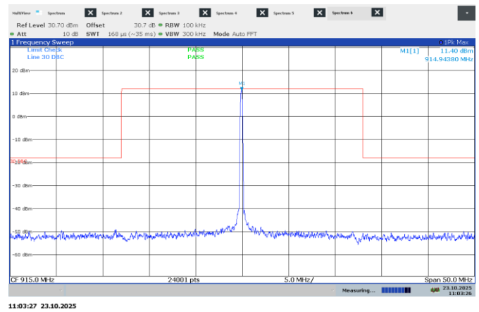
Figure 7.8-8: Conducted non-restricted band edge emissions at 928 MHz
