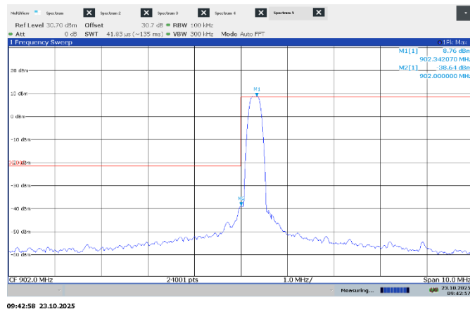
Figure 7.8-7: Conducted non-restricted band edge emissions at 902 MHz
