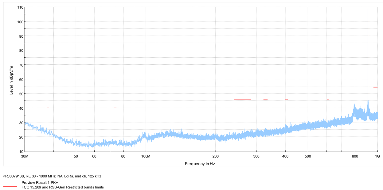
Figure 7.8-2: Radiated spurious emissions 30-1000 MHz mid channel
