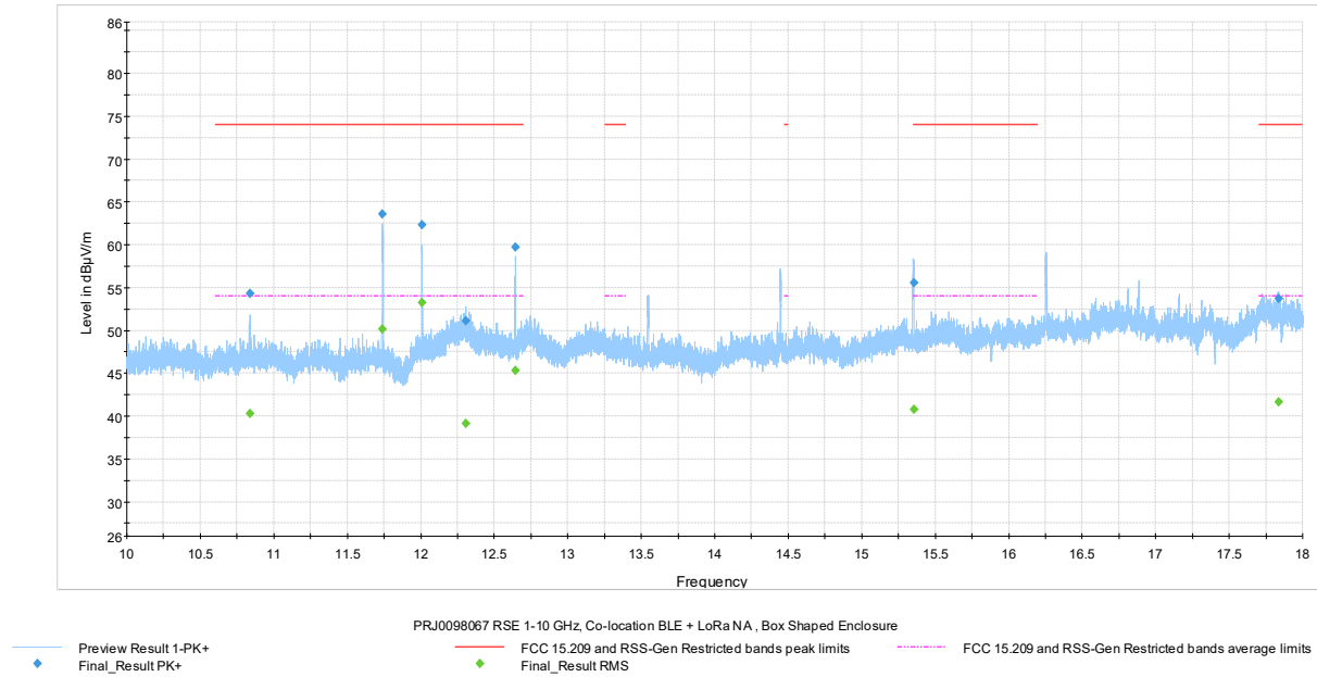
Figure 7.8-26: Radiated spurious emissions 10-18 GHz, Pulse Mouse iQ TOTAL
