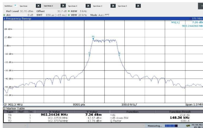
Figure 7.4-1: 20 dB bandwidth on low channel
