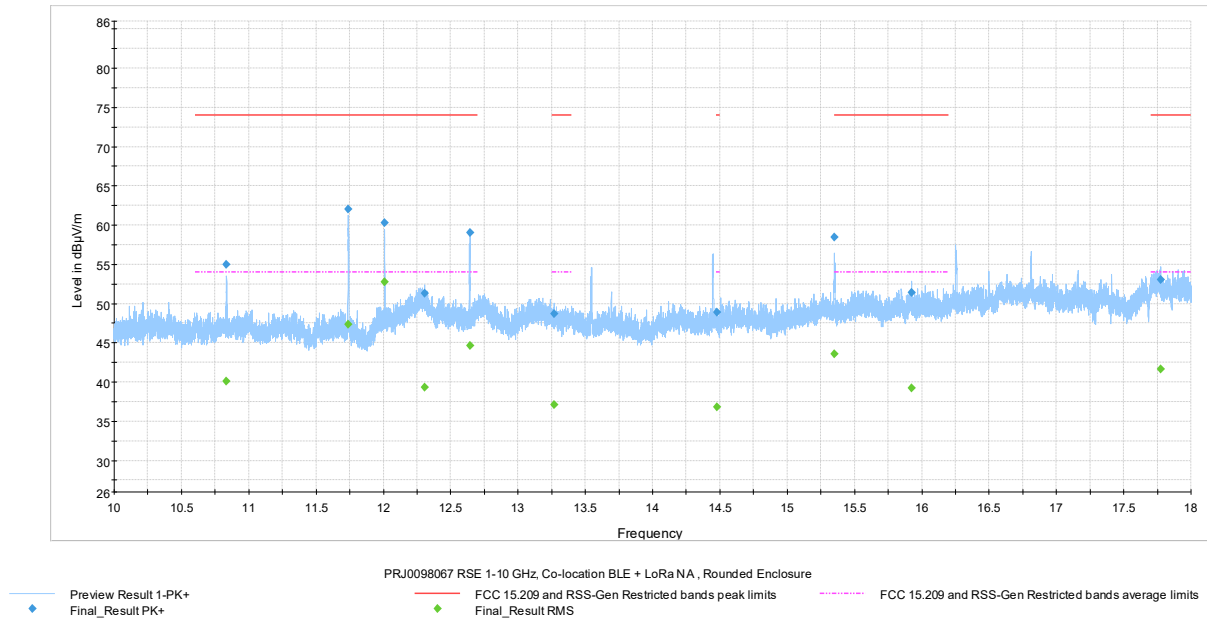
Figure 7.8-21: Radiated spurious emissions 10-18 GHz, Pulse Rat iQ TOTAL
