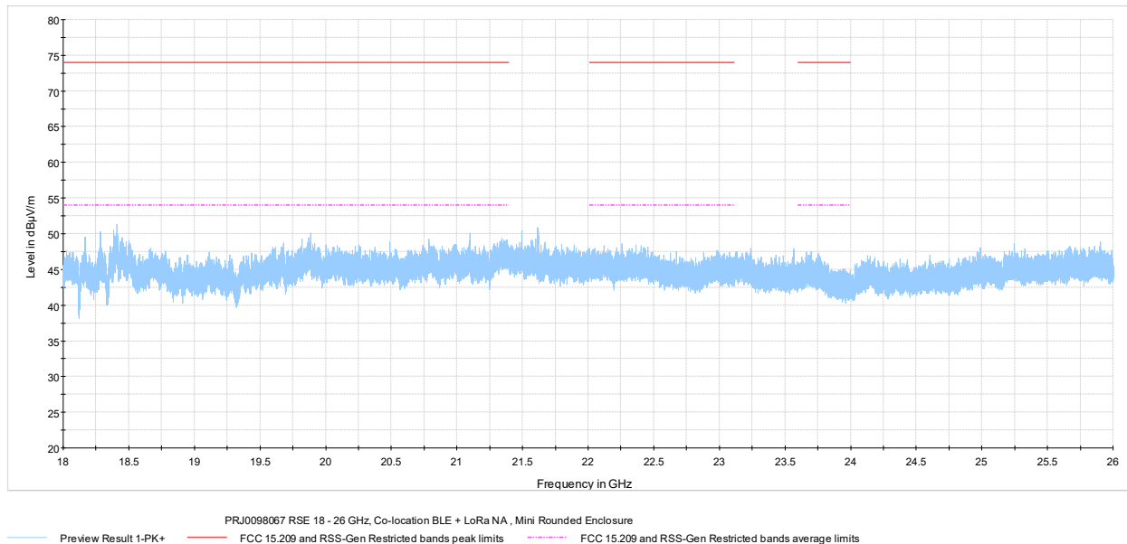
Figure 7.8-32: Radiated spurious emissions 18-26 GHz, 24/7 iQ TOTAL
