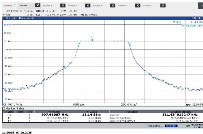
Figure 7.6-5: 99% occupied bandwidth on mid ch, 500 kHz bandwidth signal
