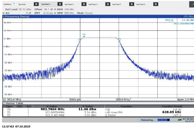
Figure 7.6-1: 6 dB bandwidth on low ch, 500 kHz bandwidth signal
