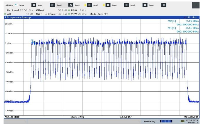
Figure 7.4-4: Carrier frequency separation
