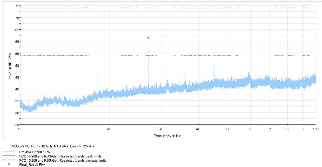
Figure 7.8-4: Radiated spurious emissions 1-10 GHz low channel
