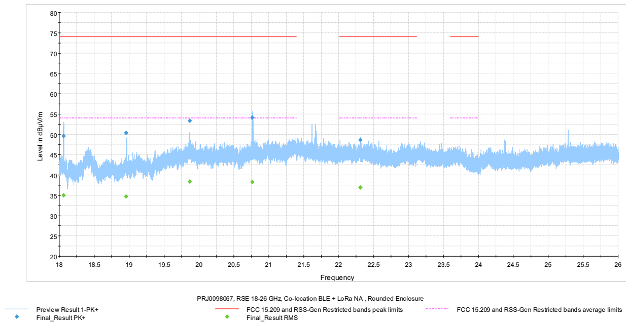
Figure 7.8-22: Radiated spurious emissions 18-26 GHz, Pulse Rat iQ TOTAL
