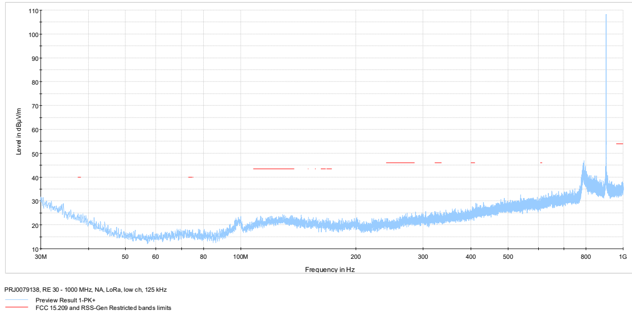
Figure 7.8-1: Radiated spurious emissions 30-1000 MHz low channel
