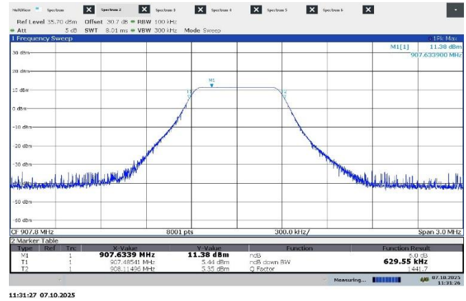
Figure 7.6-2: 6 dB bandwidth on mid ch, 500 kHz bandwidth signal
