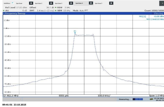
Figure 7.9-1: PSD on low channel, 125 kHz signal
