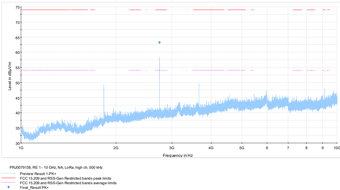
Figure 7.8-15: Radiated spurious emissions 1-10 GHz high channel
