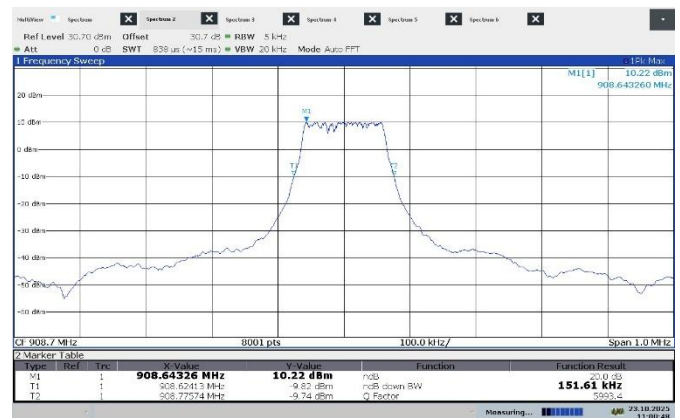
Figure 7.4-2: 20 dB bandwidth on mid channel
