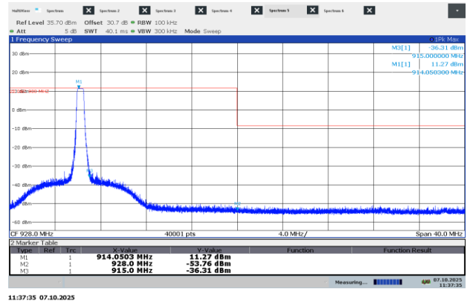
Figure 7.8-17: Conducted non-restricted band edge emissions at 928 MHz
