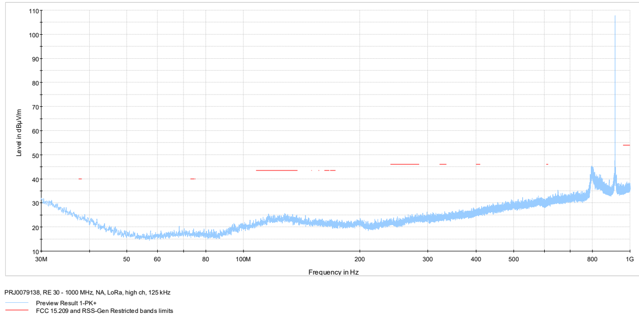
Figure 7.8-3: Radiated spurious emissions 30-1000 MHz high channel
