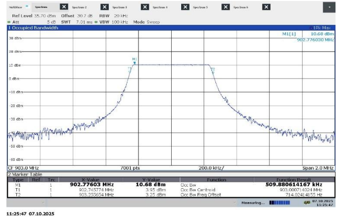
Figure 7.6-4: 99% occupied bandwidth on low ch, 500 kHz bandwidth signal
