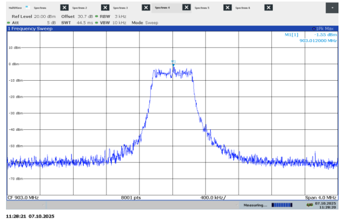
Figure 7.9-4: PSD on low channel, 500 kHz signal
