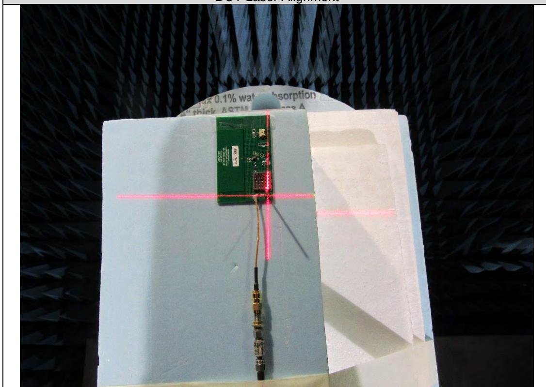
DUT Laser Alignment
