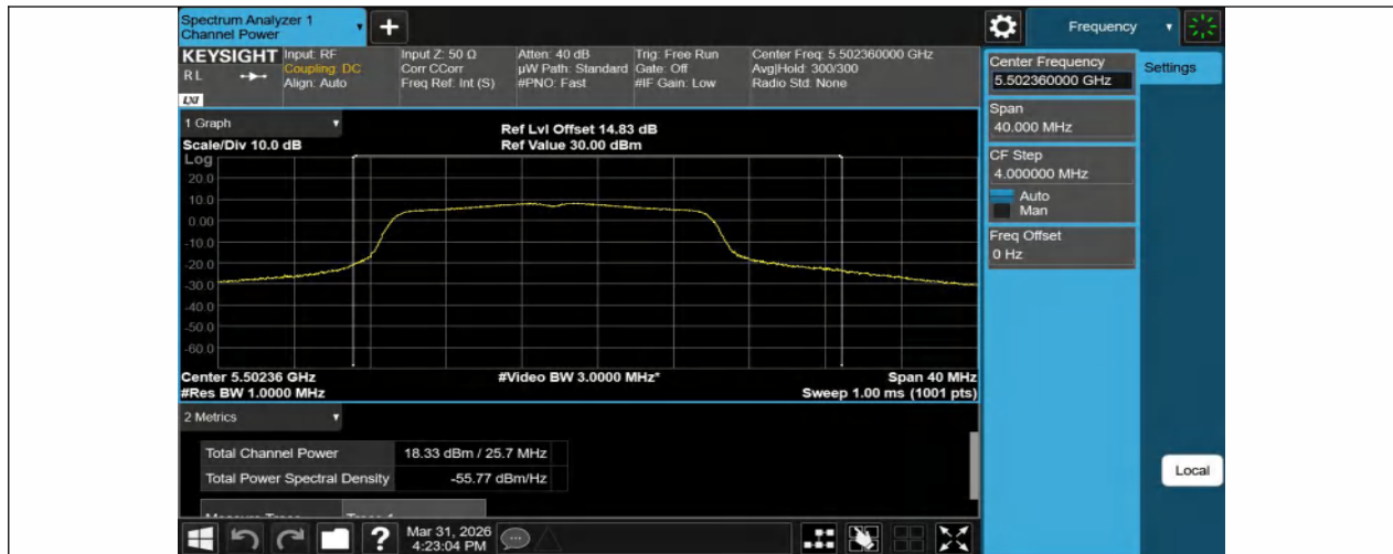
11A-Ant1-5500-PASS
