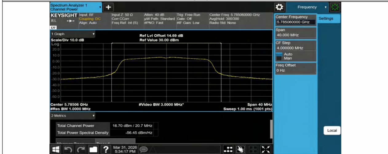
11A-Ant1-5785-PASS
