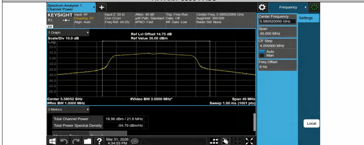
11A-Ant1-5580-PASS
