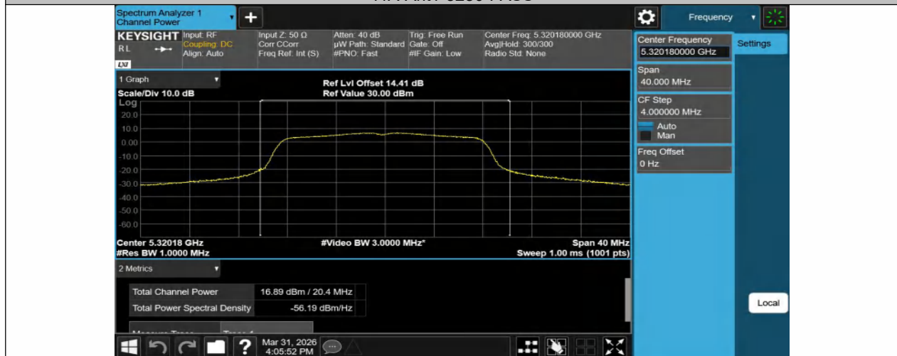
11A-Ant1-5320-PASS
