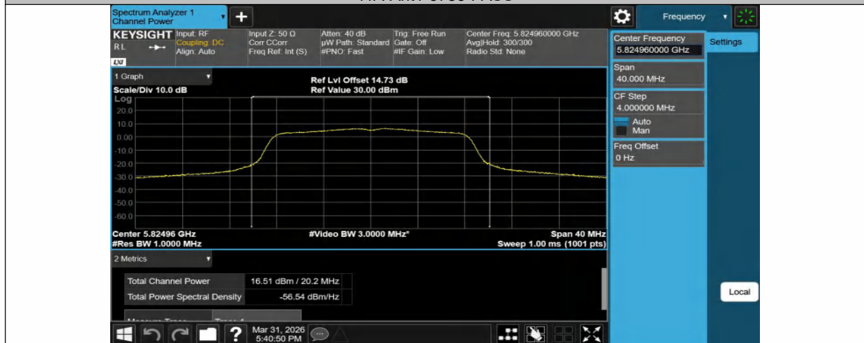
11A-Ant1-5825-PASS
