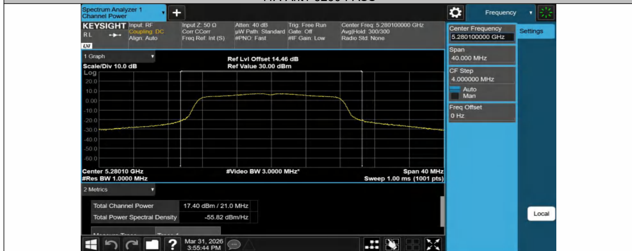
11A-Ant1-5280-PASS
