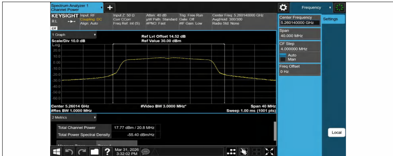
11A-Ant1-5260-PASS
