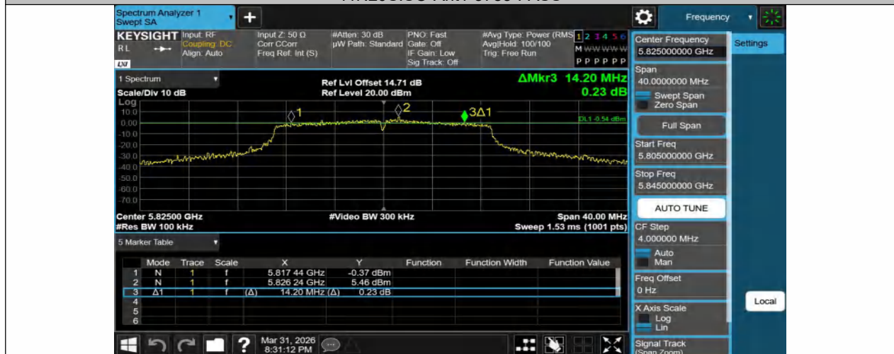
11N20SISO-Ant1-5825-PASS
