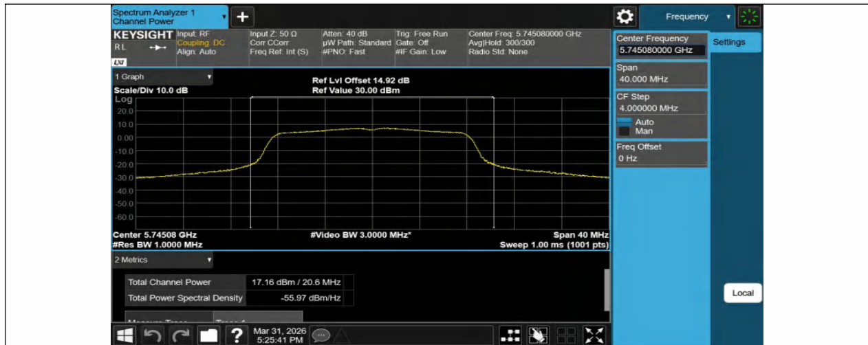
11A-Ant1-5745-PASS
