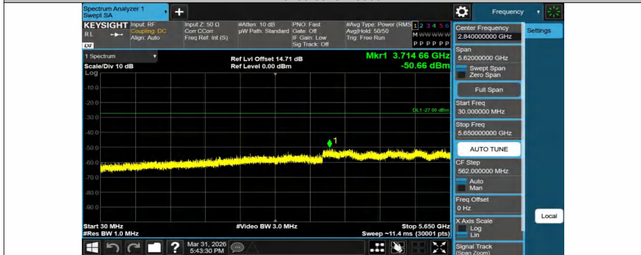
11A-Ant1-5825-30~5650-PASS
