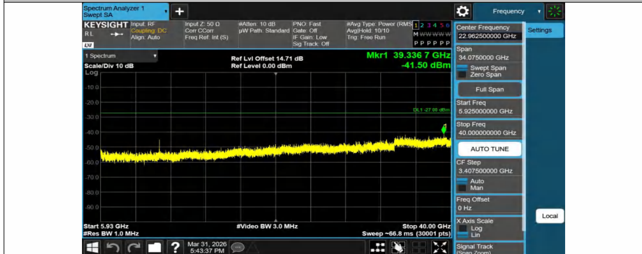
11A-Ant1-5825-5925~40000-PASS
