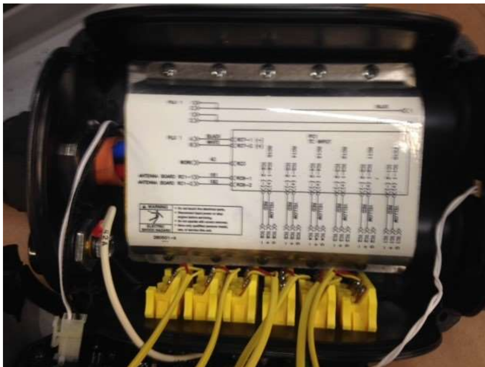
Interior photo of the Box open:
