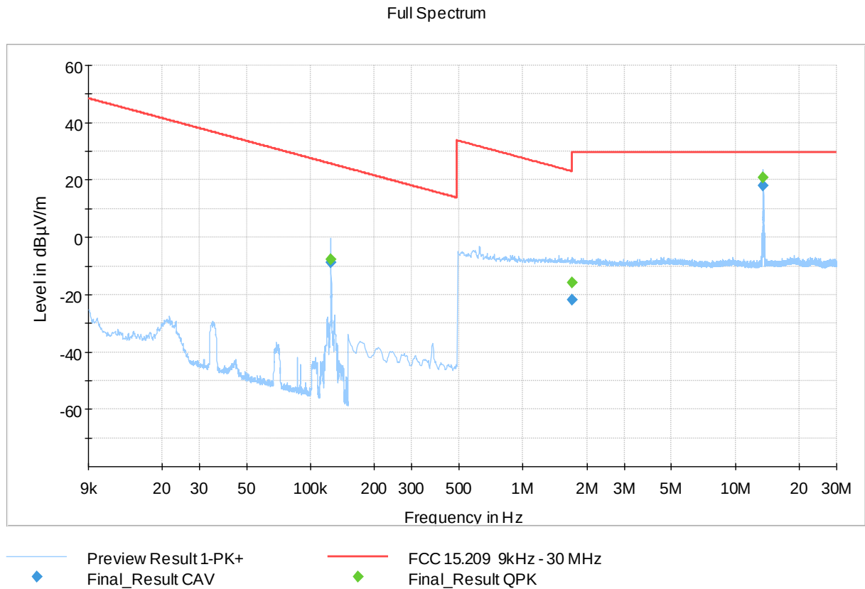
Figure 3: TX radiated emission 9 kHz to 30MHz
