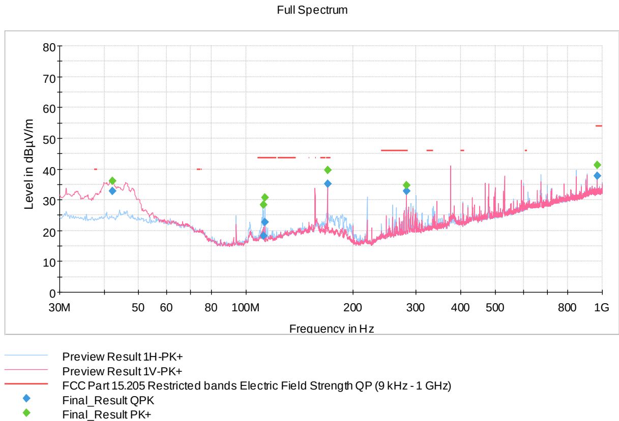
Figure 4: TX radiated emission 30 – 1000 MHz
