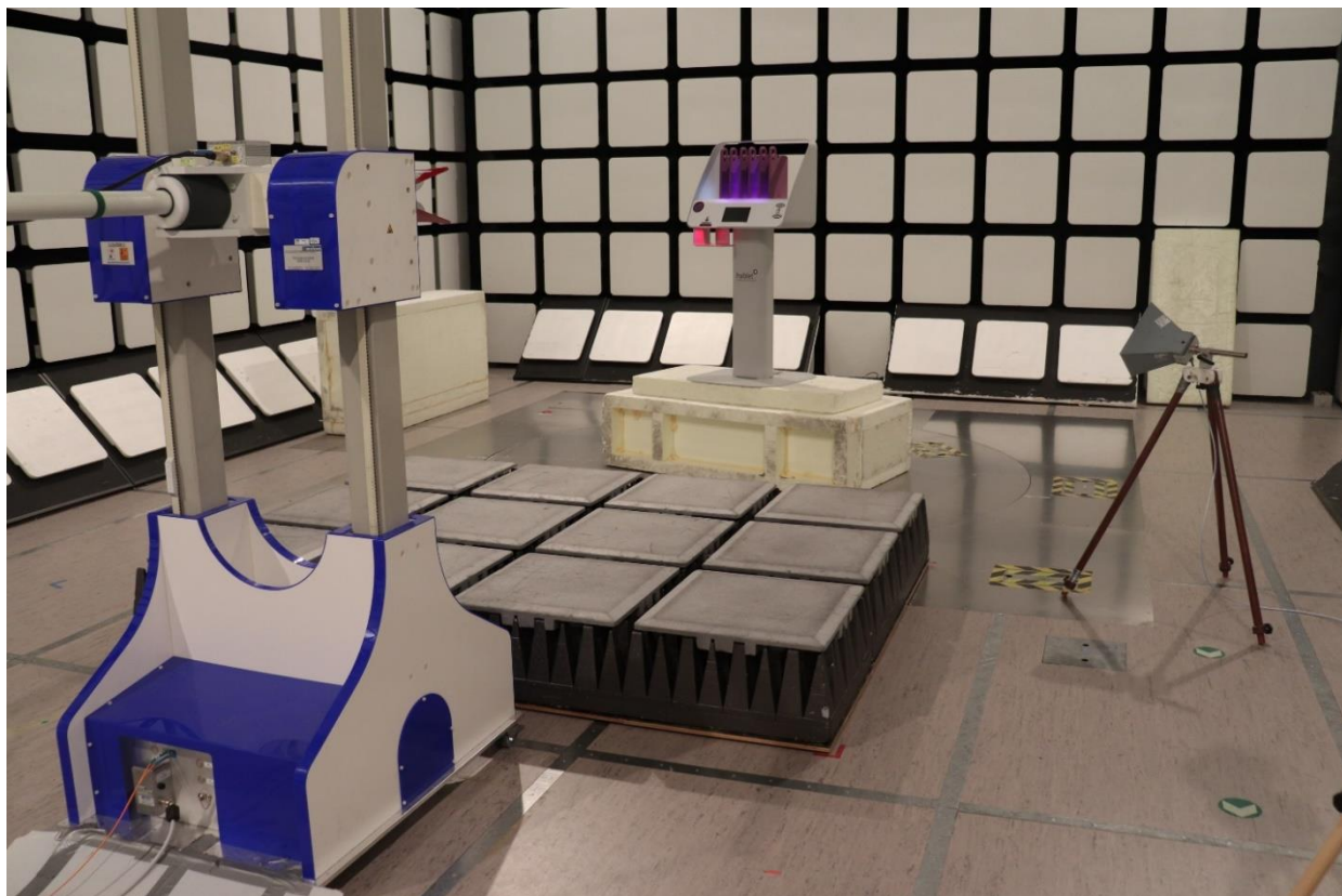
Photograph 2: Radiated emissions (1 – 18 GHz)
