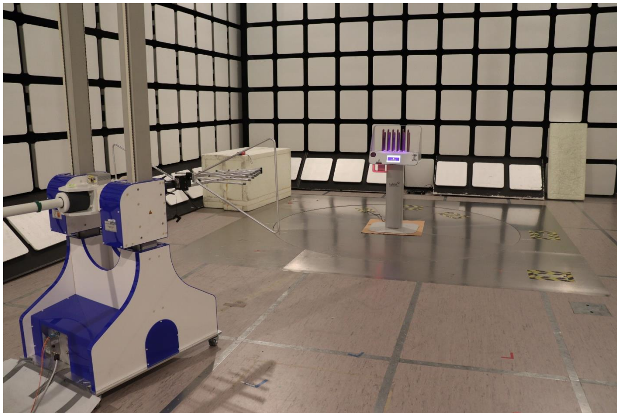
Photograph 1: Radiated emissions (30 – 1000 MHz)
