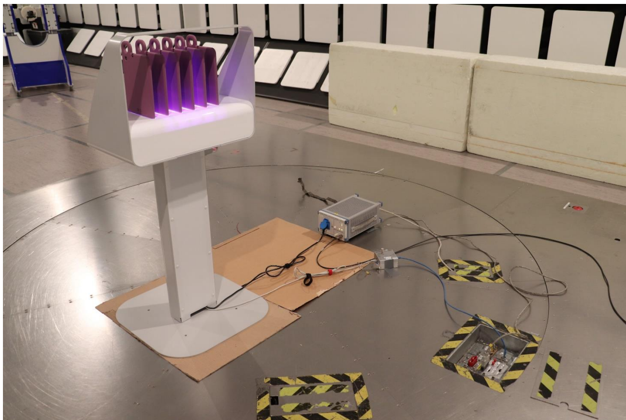
Photograph 3: Conducted emissions (0.150 – 30 MHz)
