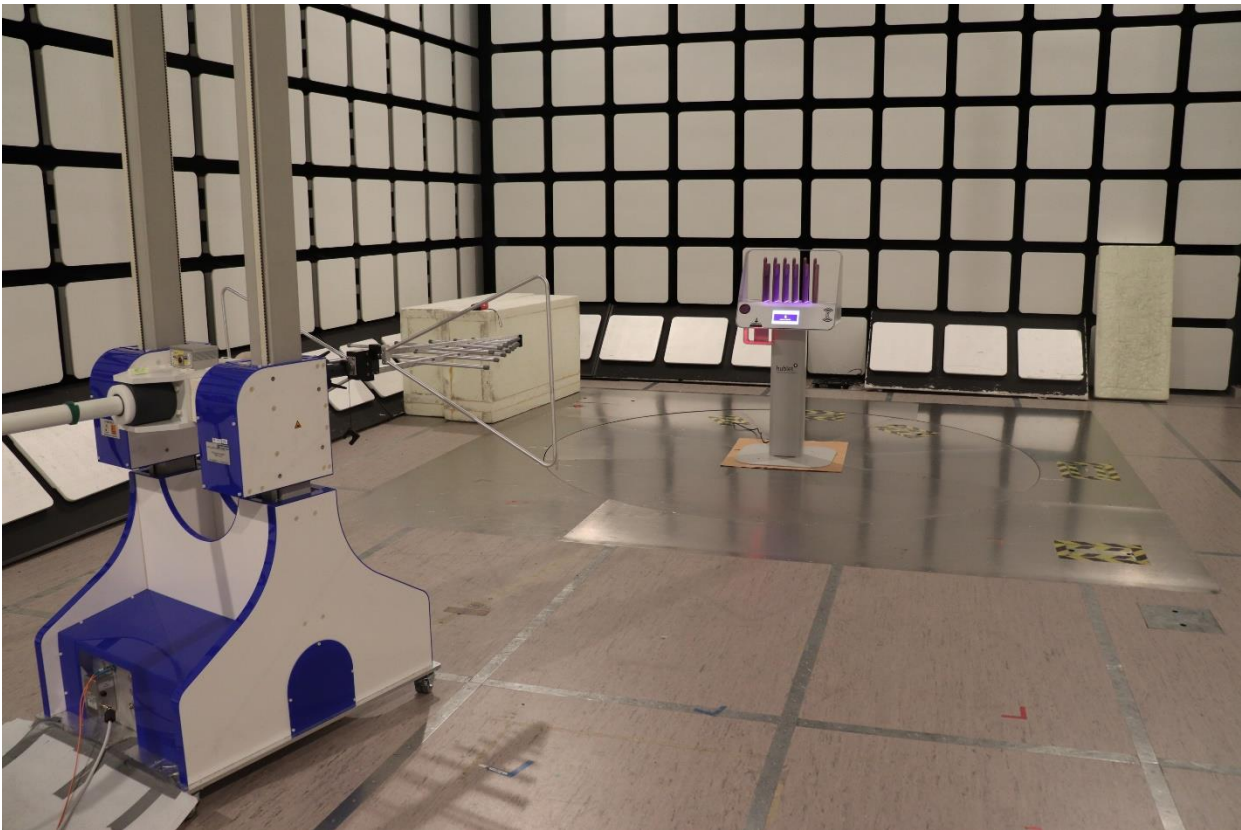
Photograph 1: Transmitter radiated emissions in restricted bands (30 – 1000 MHz)
