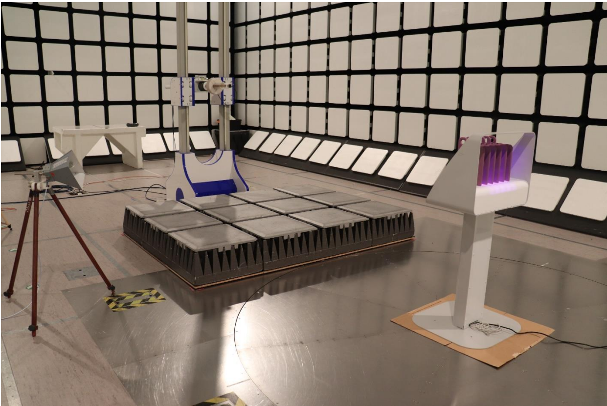
Photograph 3: Transmitter radiated emissions in restricted bands (18 – 26.5 GHz)
