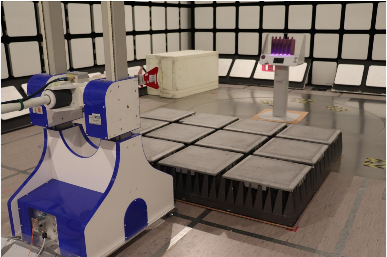
Photograph 2: Transmitter radiated emissions in restricted bands (1 – 18 GHz)
