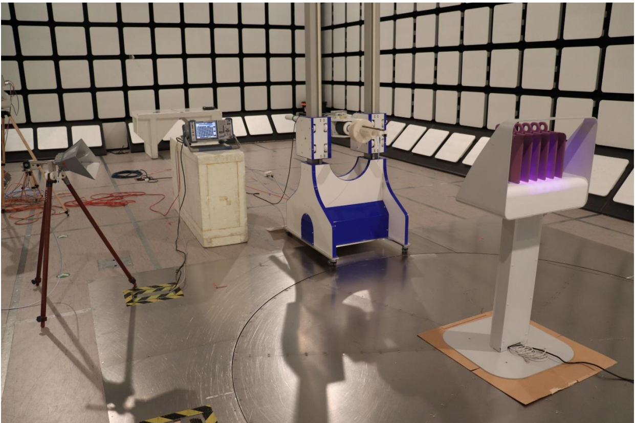
Photograph 4: Transmitter radiated emissions in restricted bands (26.5 – 40 GHz)
