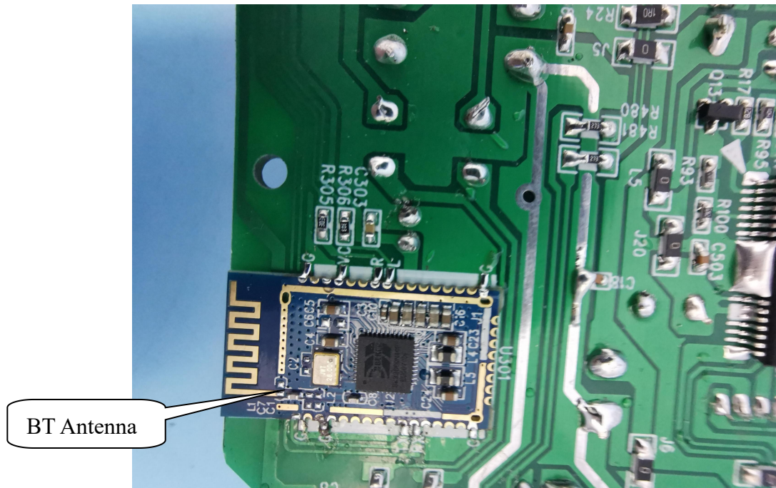
INTERNAL VIEW-4 OF EUT
