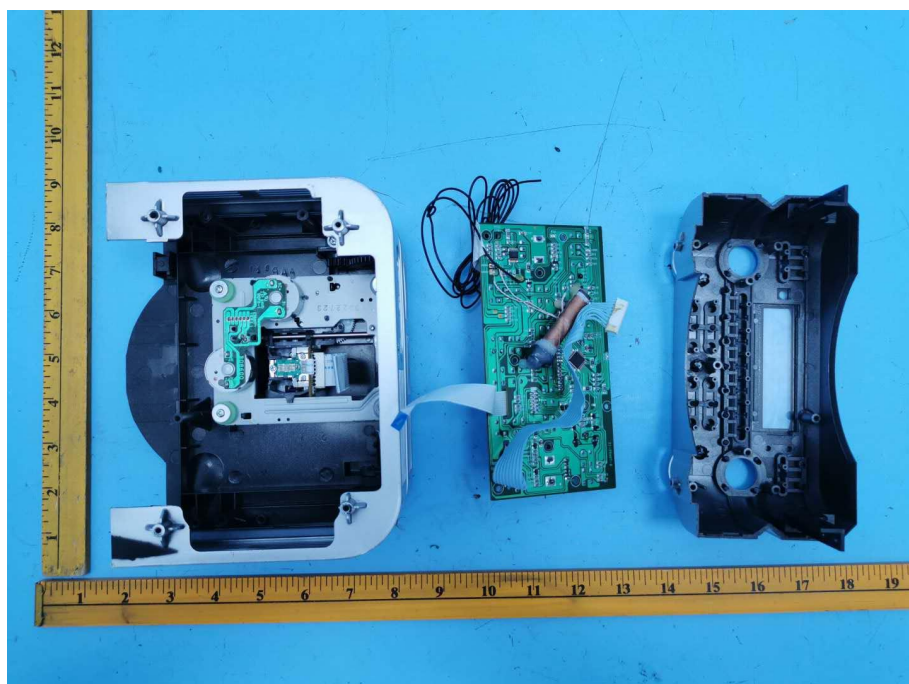
INTERNAL VIEW-5 OF EUT
