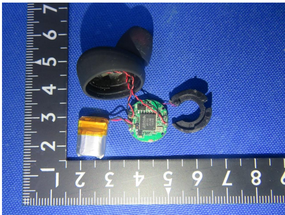
(6) EUT Photo (Right Headphone)
