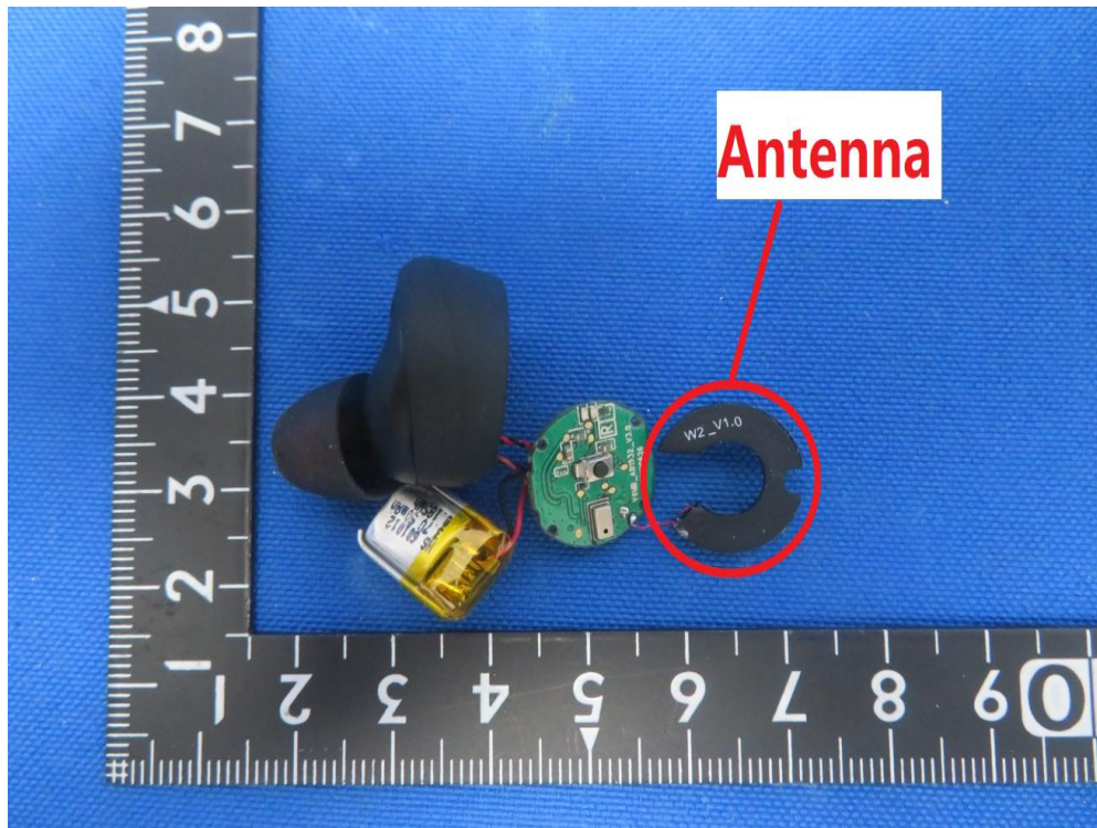
(5) EUT Photo (Right Headphone)
