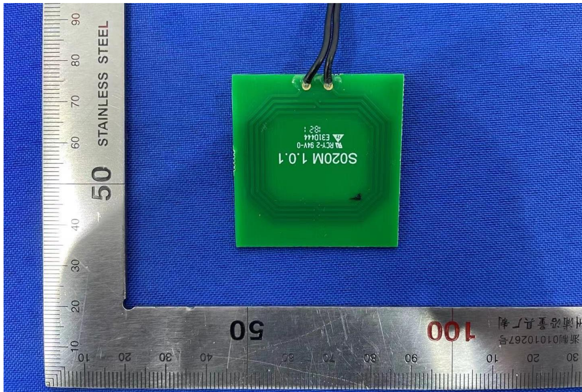
Internal 13 NFC Antenna
