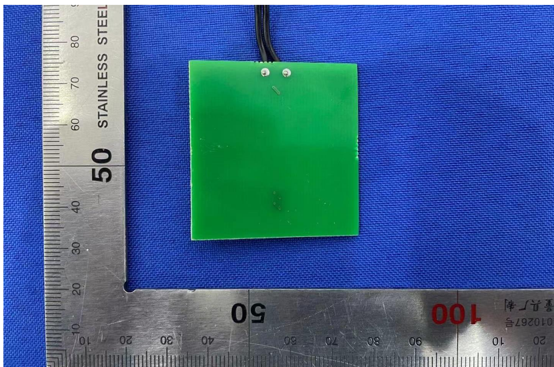
Internal 14 NFC Antenna
