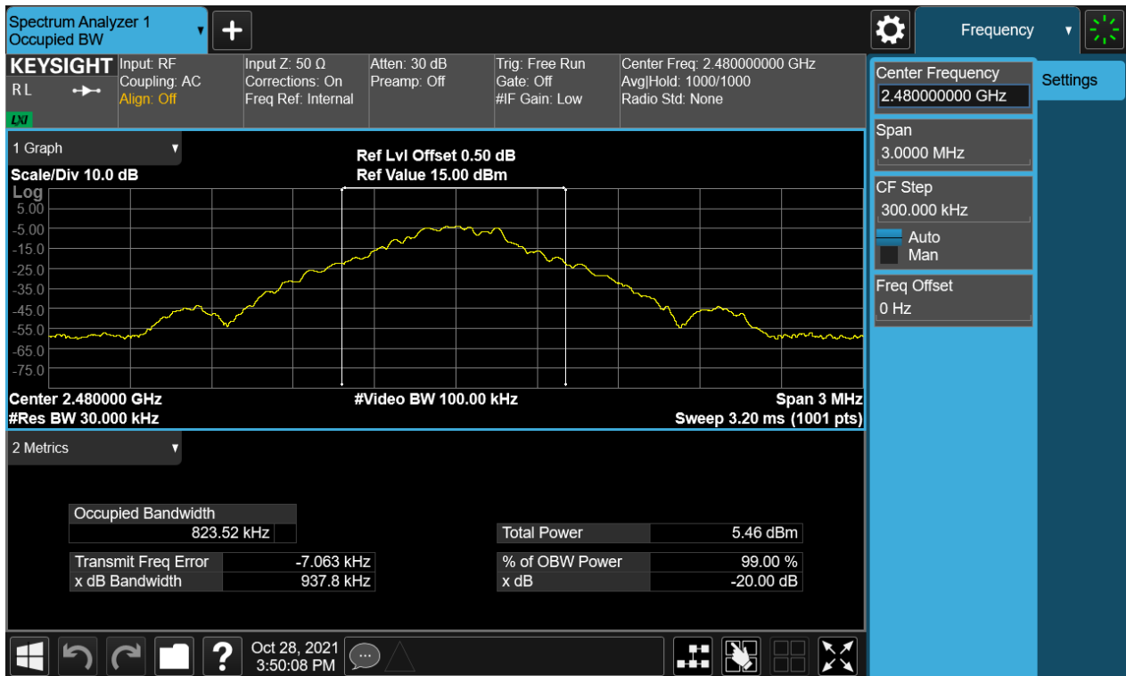
Figure 12: 20dB Bandwidth and 99% Bandwidth, 2480MHz, GFSK
