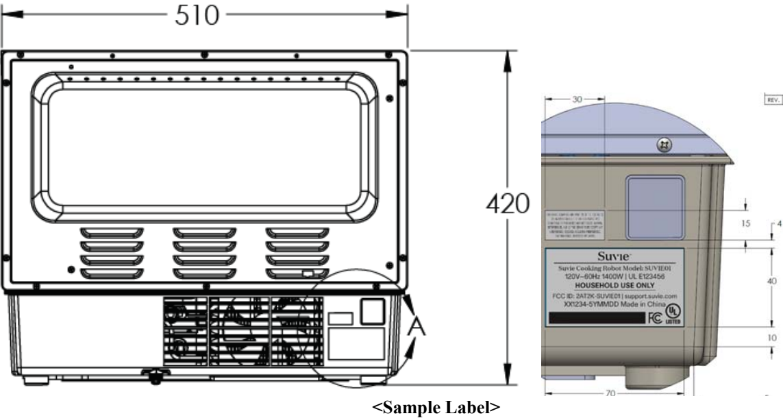
<Label Location>
