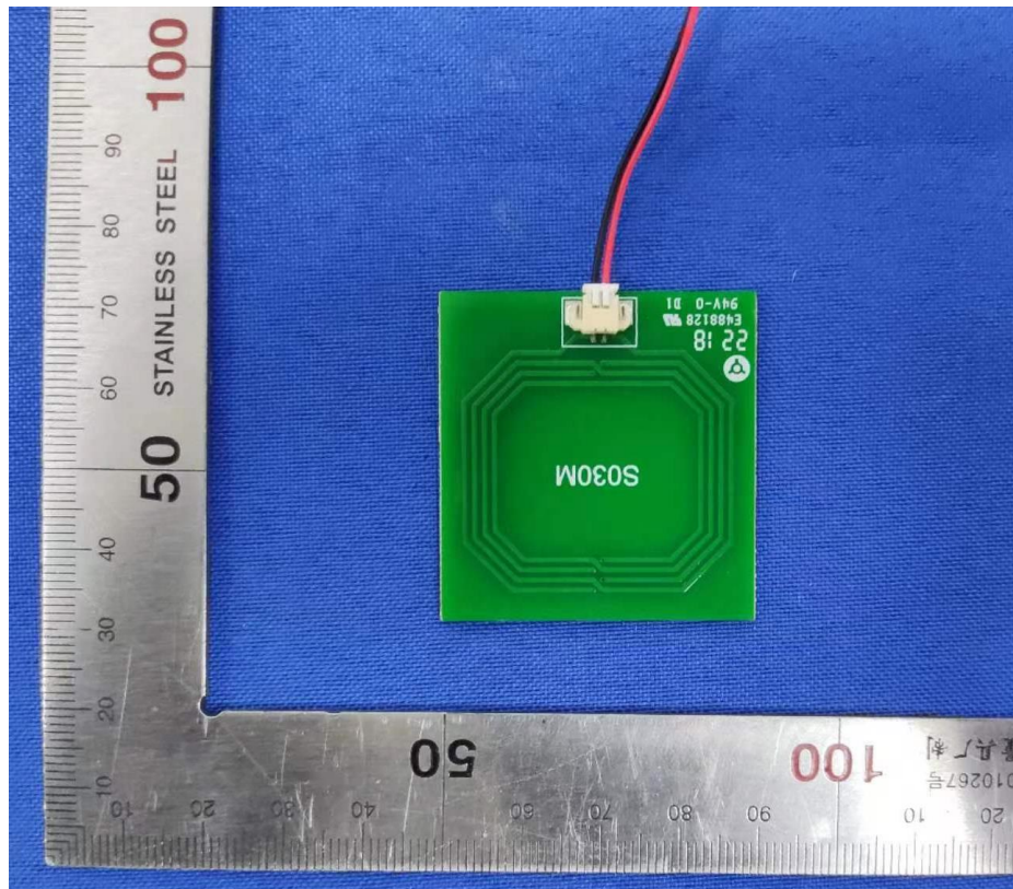
Internal 11 NFC Antenna
