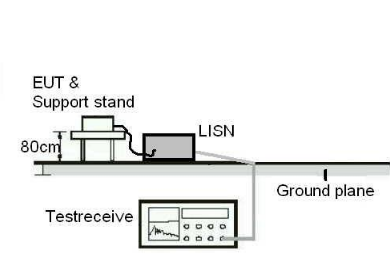
Diagram of Measurement Configuration for Conduction Test
