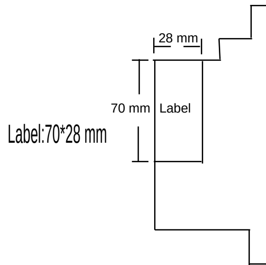
LEFT VIEW(Bluetooth Controller)
