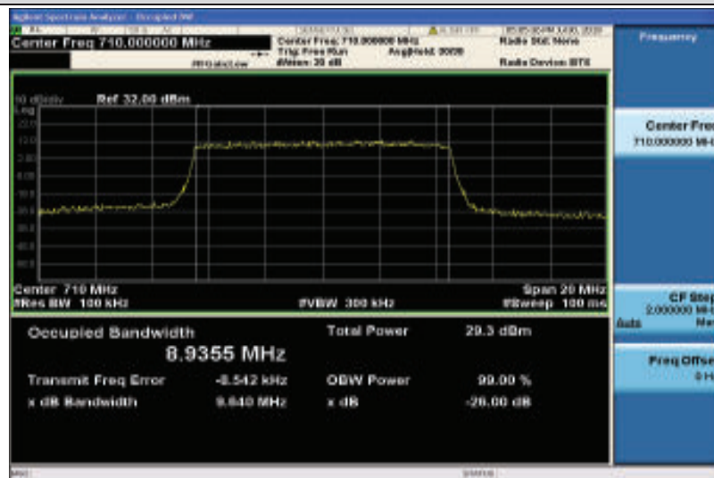
Band17-10MHz-QPSK-23790-50RB#0-8.9355
