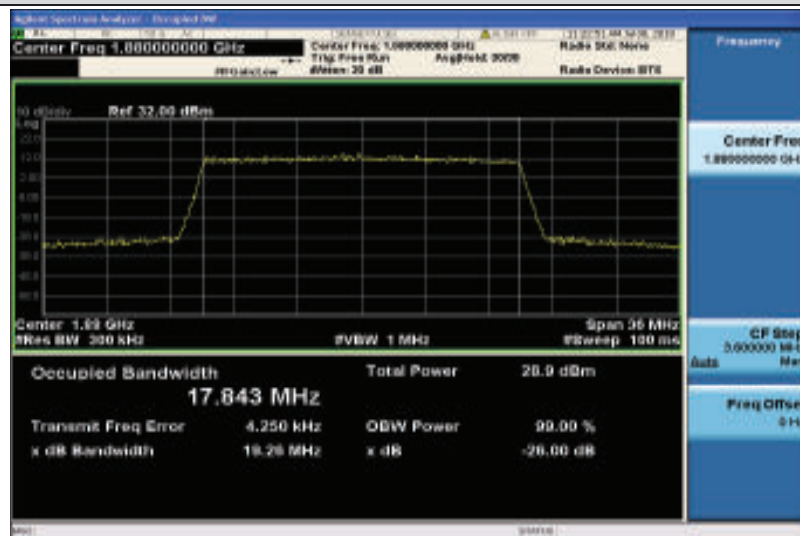
Band2-20MHz-16QAM-18900-100RB#0-17.843
