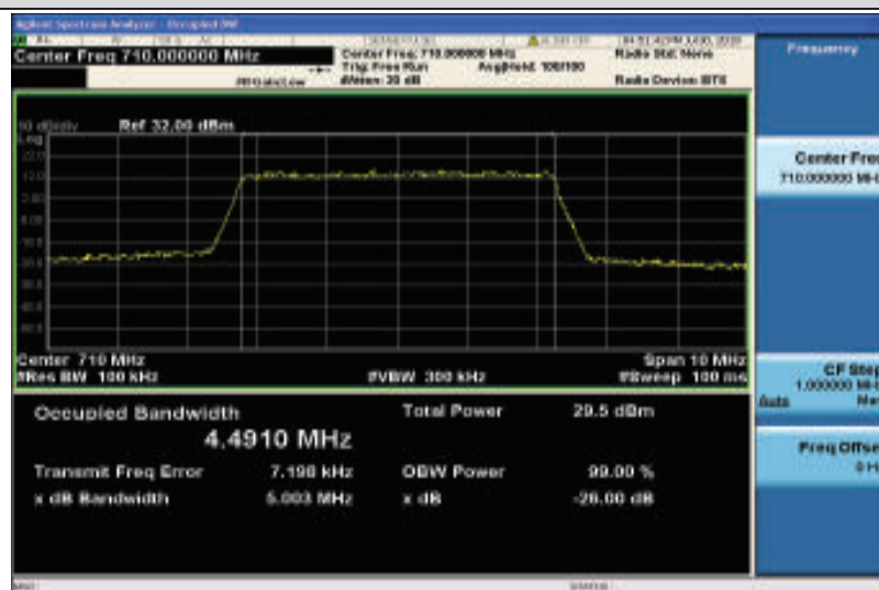
Band17-5MHz-QPSK-23790-25RB#0-4.4910
