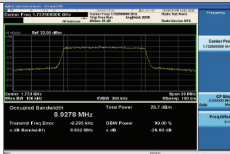
Band4-10MHz-16QAM-20175-50RB#0-8.9278
