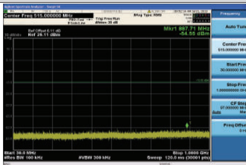
Band2-15MHz-16QAM-19125-1RB#0-30~1000MHz
