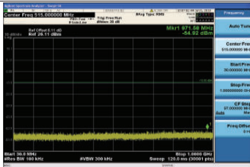
Band4-3MHz-16QAM-19965-1RB#0-30~1000MHz
