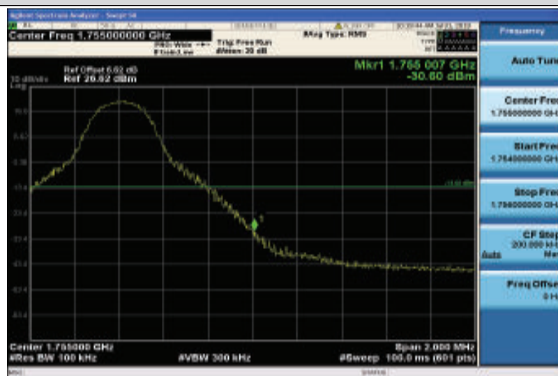
Band4-10MHz-QPSK-20350-1RB#49
