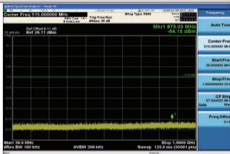
Band4-3MHz-16QAM-20385-1RB#0-30~1000MHz
