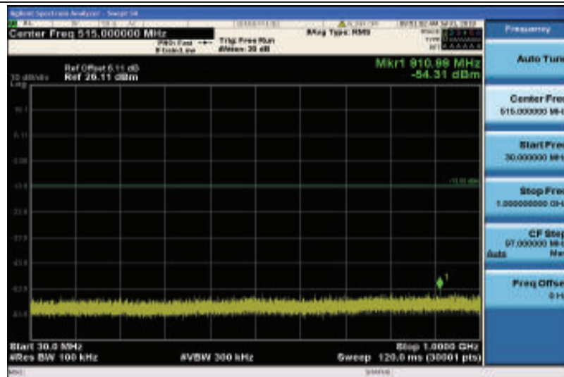
Band2-15MHz-16QAM-18900-1RB#0-30~1000MHz
