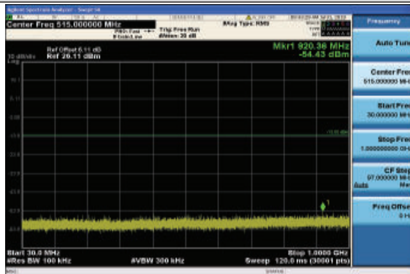
Band2-10MHz-16QAM-18650-1RB#0-30~1000MHz
