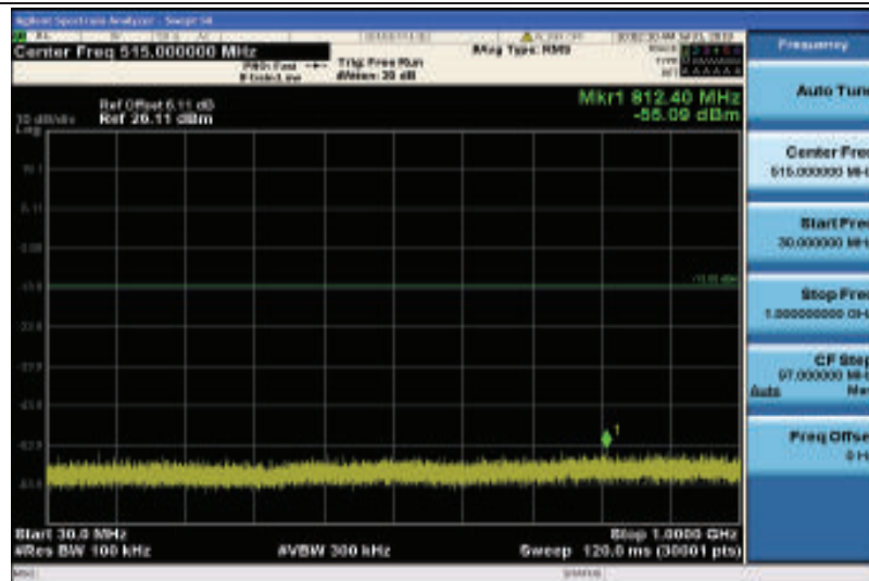
Band4-1.4MHz-16QAM-20175-1RB#0-30~1000MHz
