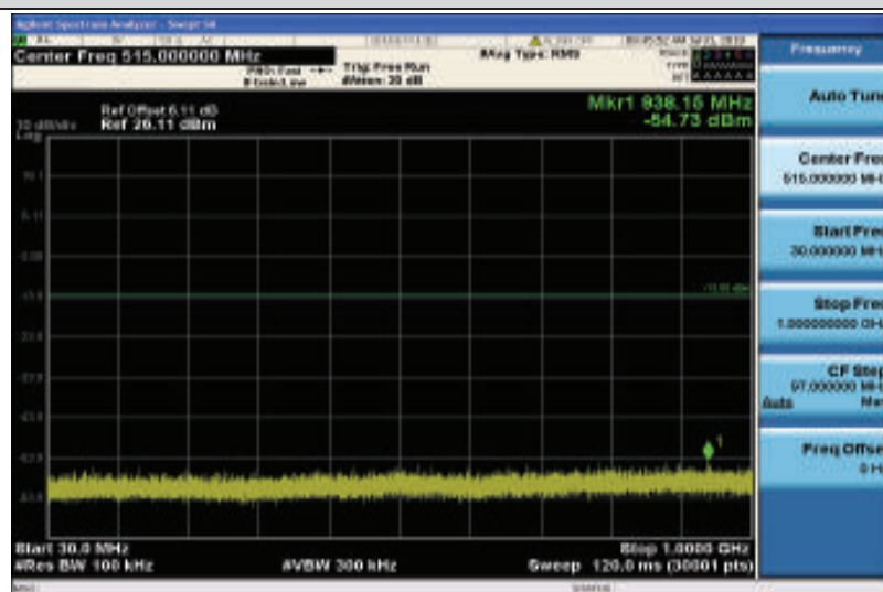
Band2-10MHz-16QAM-19150-1RB#0-30~1000MHz
