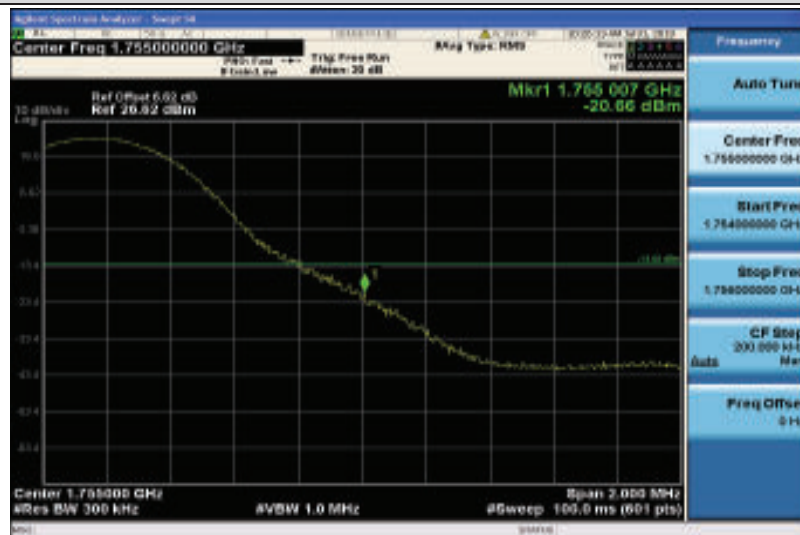
Band4-15MHz-QPSK-20325-1RB#74
