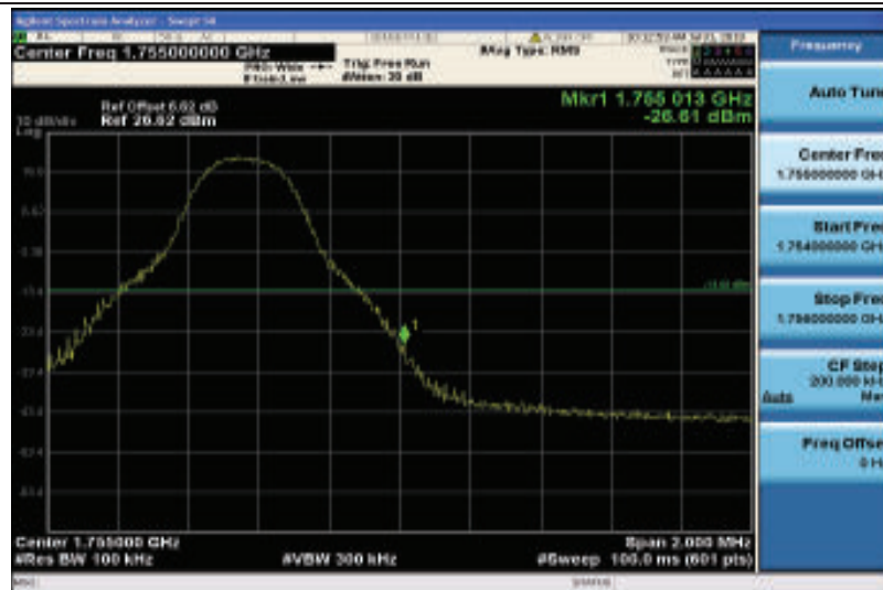
Band4-5MHz-QPSK-20375-1RB#24
