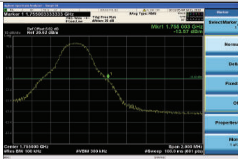
Band4-5MHz-16QAM-20375-1RB#24
