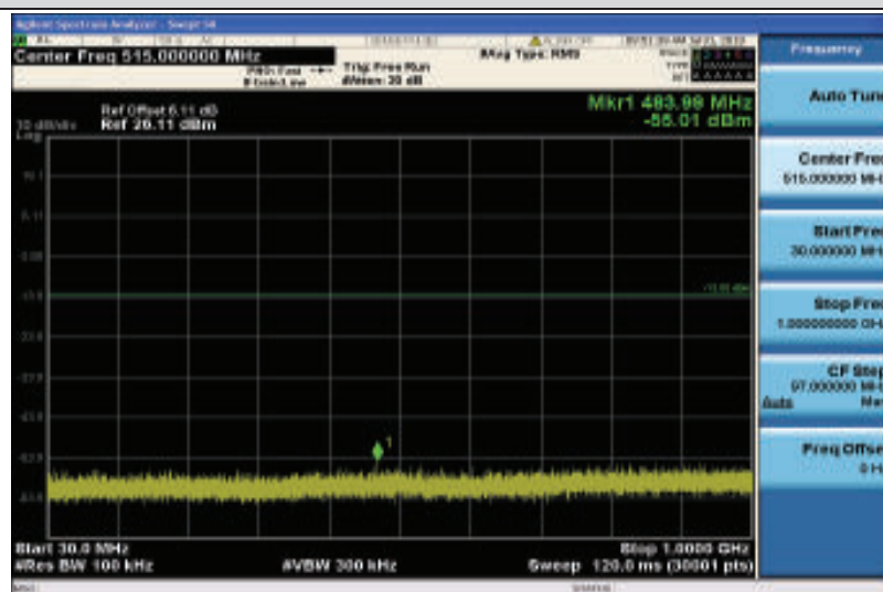
Band2-15MHz-QPSK-19125-1RB#0-30~1000MHz
