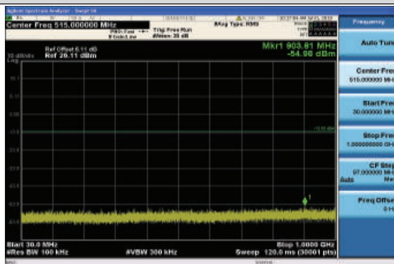
Band4-5MHz-16QAM-20375-1RB#0-30~1000MHz
