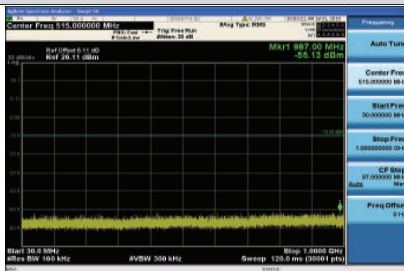
Band4-1.4MHz-16QAM-20393-1RB#0-30~1000MHz
