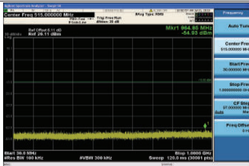
Band4-1.4MHz-16QAM-19957-1RB#0-30~1000MHz
