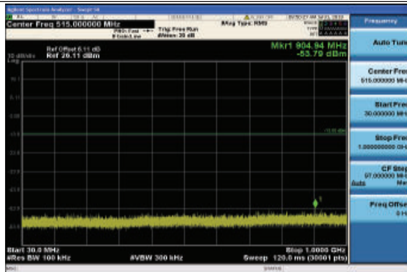
Band2-15MHz-QPSK-18900-1RB#0-30~1000MHz
