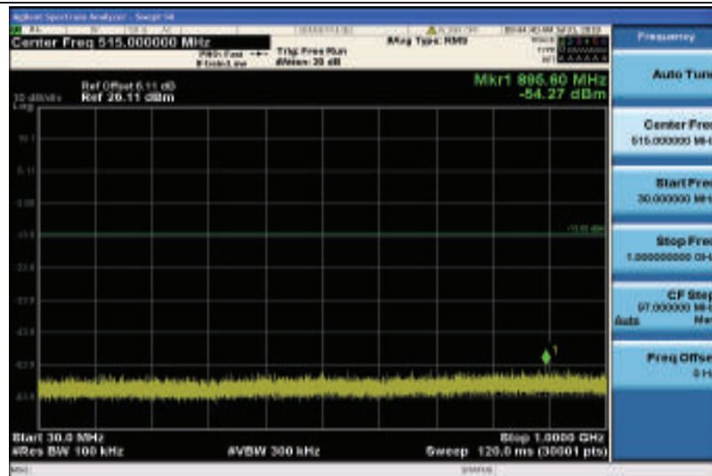
Band2-10MHz-16QAM-18900-1RB#0-30~1000MHz
