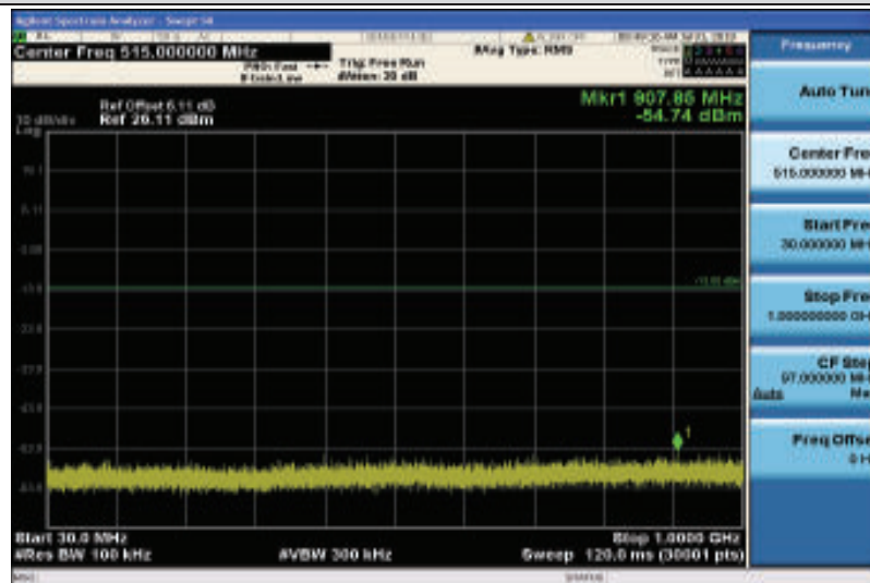
Band2-15MHz-QPSK-18675-1RB#0-30~1000MHz
