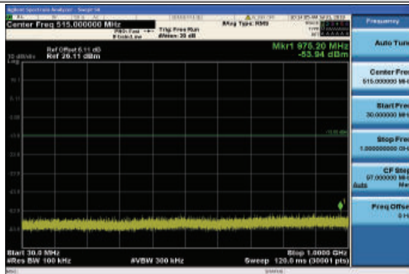
Band4-5MHz-QPSK-19975-1RB#0-30~1000MHz
