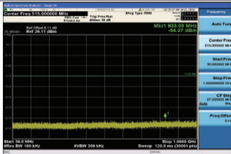
Band4-5MHz-QPSK-20175-1RB#0-30~1000MHz
