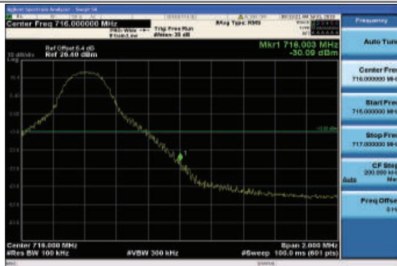
Band17-10MHz-QPSK-23800-1RB#49
