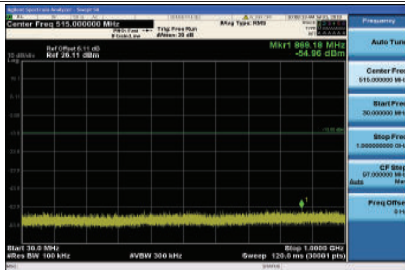
Band4-3MHz-16QAM-20175-1RB#0-30~1000MHz
