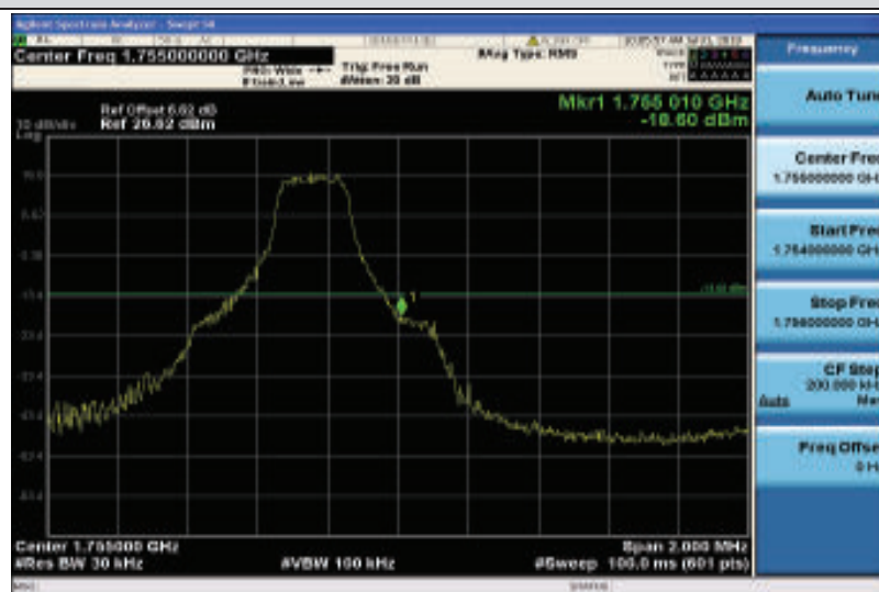
Band4-3MHz-16QAM-20385-1RB#14
