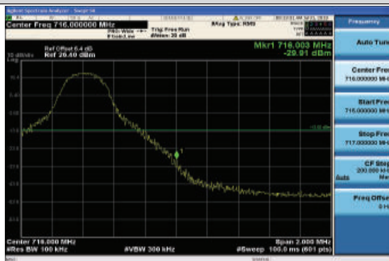
Band17-10MHz-16QAM-23800-1RB#49
