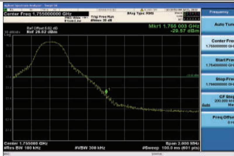
Band4-10MHz-16QAM-20350-1RB#49
