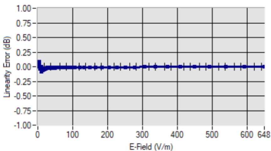
Linearity
