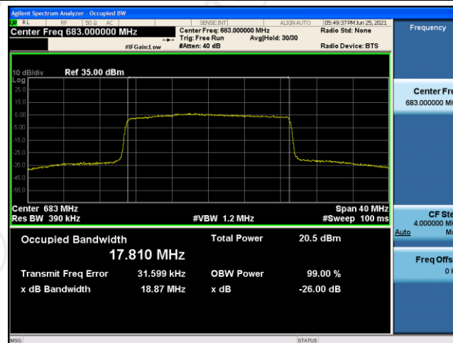
Band71-20MHz-16QAM-133372-100RB#0
