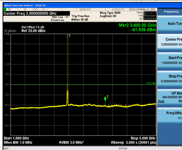
Band7-10MHz-QPSK-21400-1RB#0-Range5:5000~12000MHz
